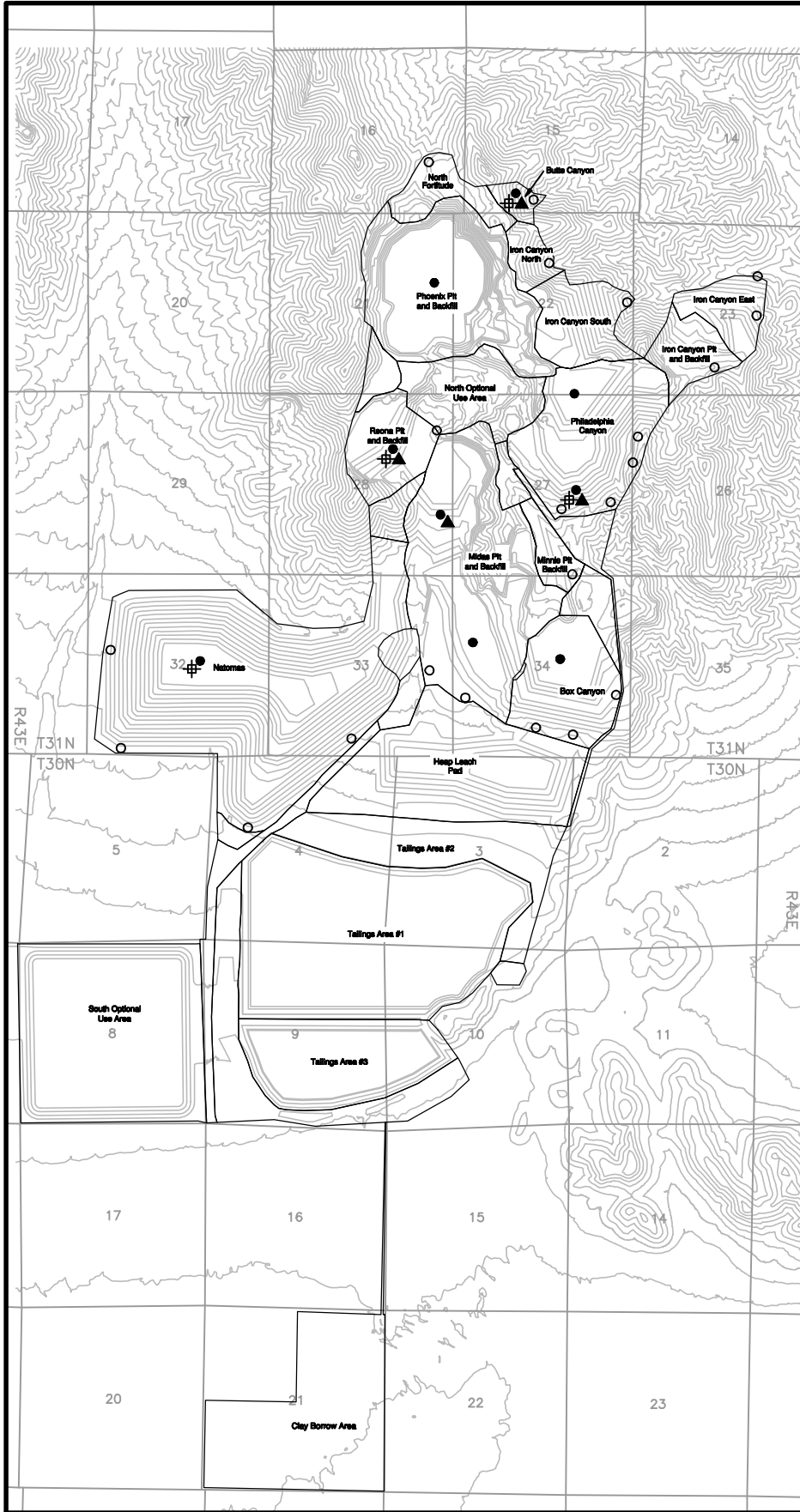
Phoenix Project Figure 3.2-29 Proposed Unsaturated Flow Monitoring Locations
