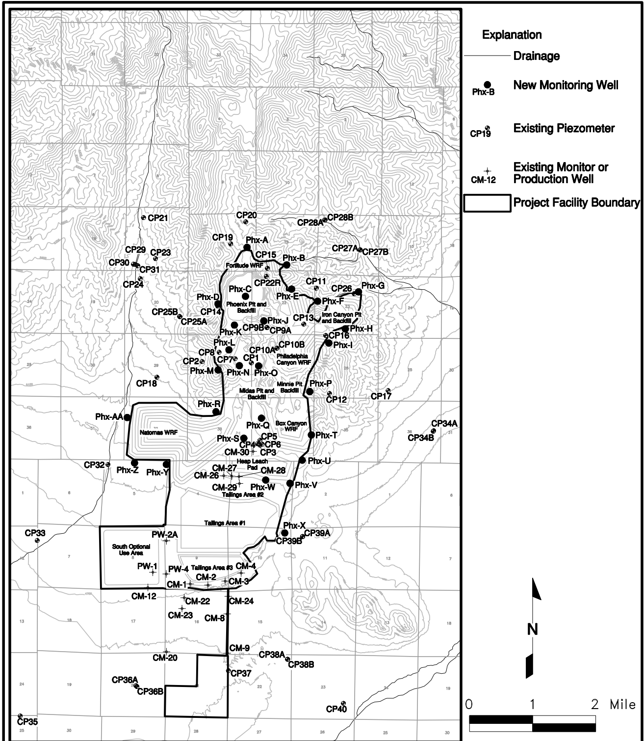
Phoenix Project Figure 3.2-28 Proposed Ground Water Monitoring Locations
