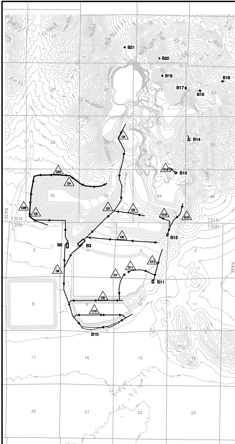
Phoenix Project Figure 3.2-19 Postreclamation Storm Water Management Design (Proposed Action)
