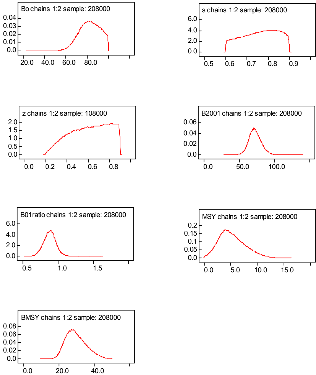
Figure 27. Posterior distributions for population parameters and management quantities for the Atlantic sharpnose shark obtained with the Bayesian LRSG model using the Gibbs sampler.
