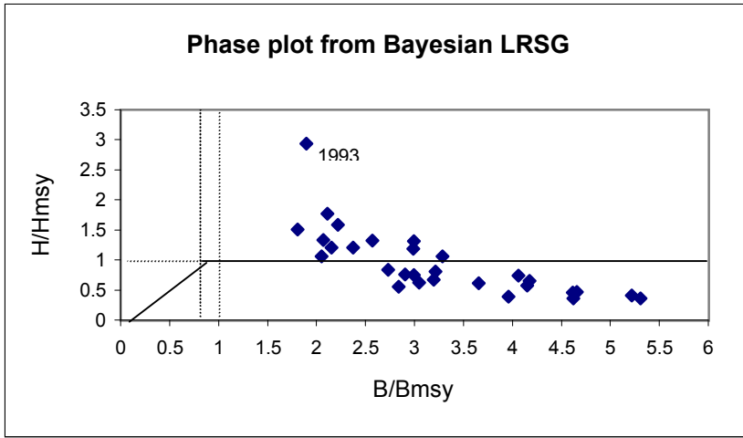
Figure 26. Phase plot and estimated trajectories of relative biomass and relative harvest rate for the small coastal shark aggregate obtained with the Bayesian LRSG using the Gibbs sampler. Values are means with 2.5th and 97.5th percentiles.
