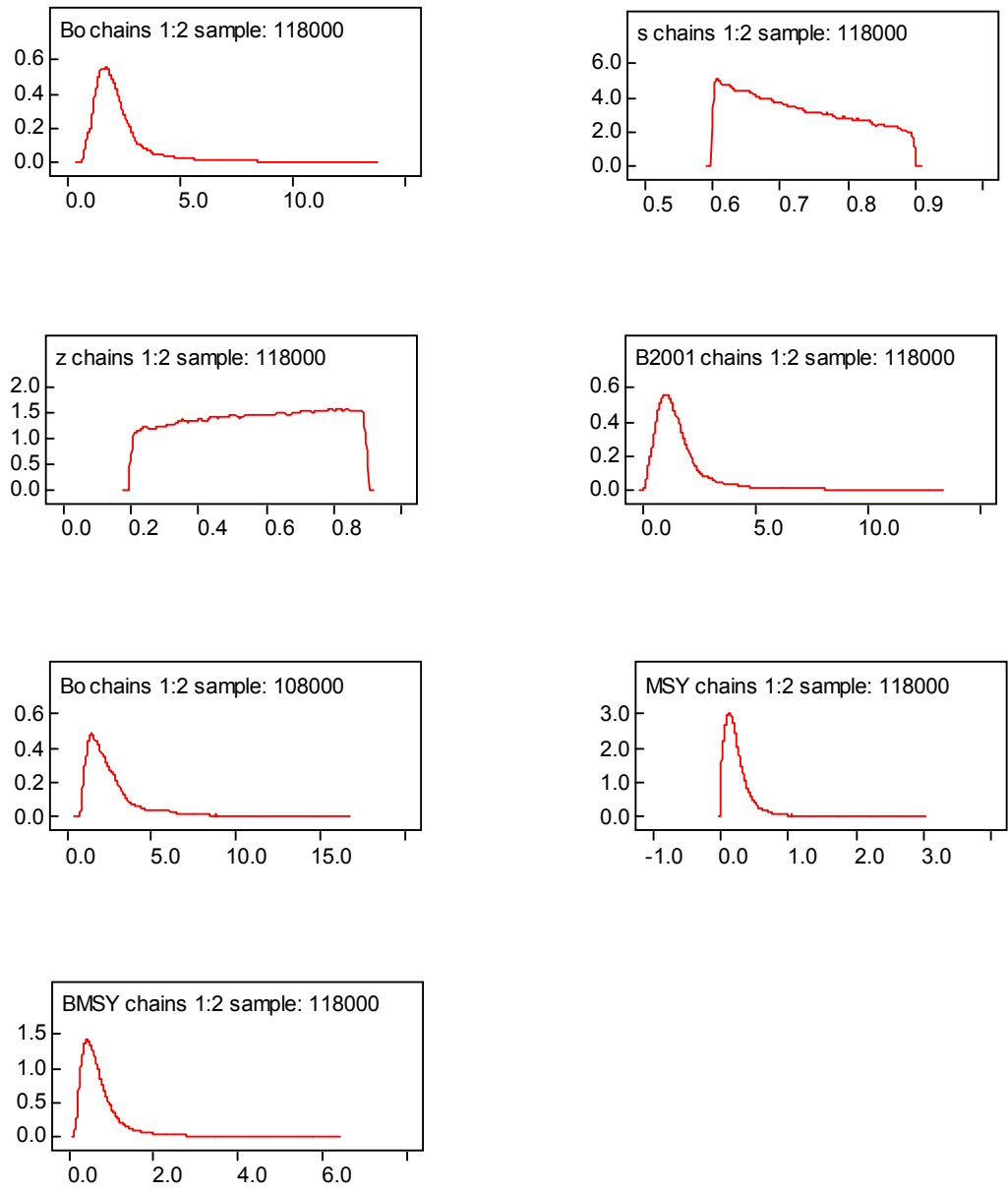
Figure 33. Posterior distributions for population parameters and management quantities for the finetooth shark obtained with the Bayesian LRSG model using the Gibbs sampler.
