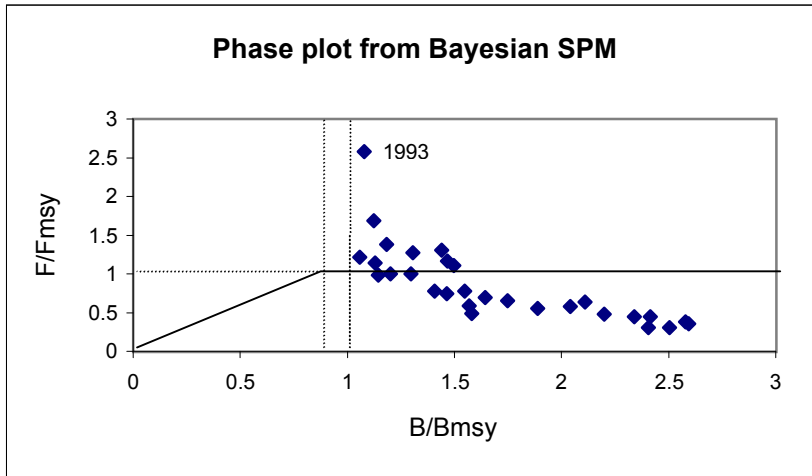
Figure 16. Phase plot and estimated trajectories of relative biomass and relative fishing mortality for the small coastal shark aggregate obtained with the Bayesian SPM using the Gibbs sampler. Values are means with 2.5th and 97.5th percentiles.
