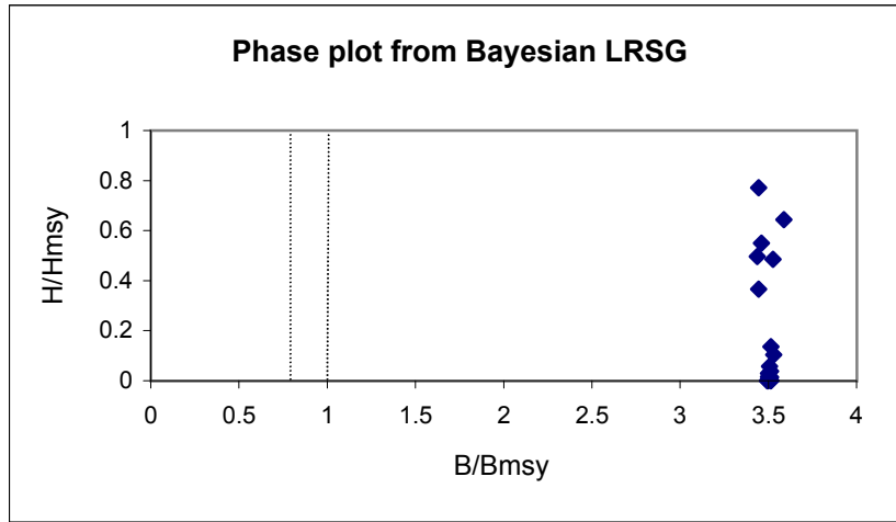
Figure 32. Phase plot and estimated trajectories of relative biomass and relative harvest rate for blacknose shark obtained with the Bayesian LRSG using the Gibbs sampler. Values are means with 2.5th and 97.5th percentiles.
