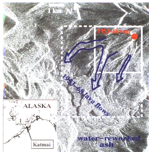
Figure 1. ERS-1 radar image of New Trident volcano and surrounding region. The location of the Katmai region with respect to Alaska is shown at the lower left corner. The location of the center of the figure is 58.20^{\circ}\text{N}/155.17^{\circ}\text{W} . The solid and dashed white polygons denote the area covered by Figures 2a and 2b.
