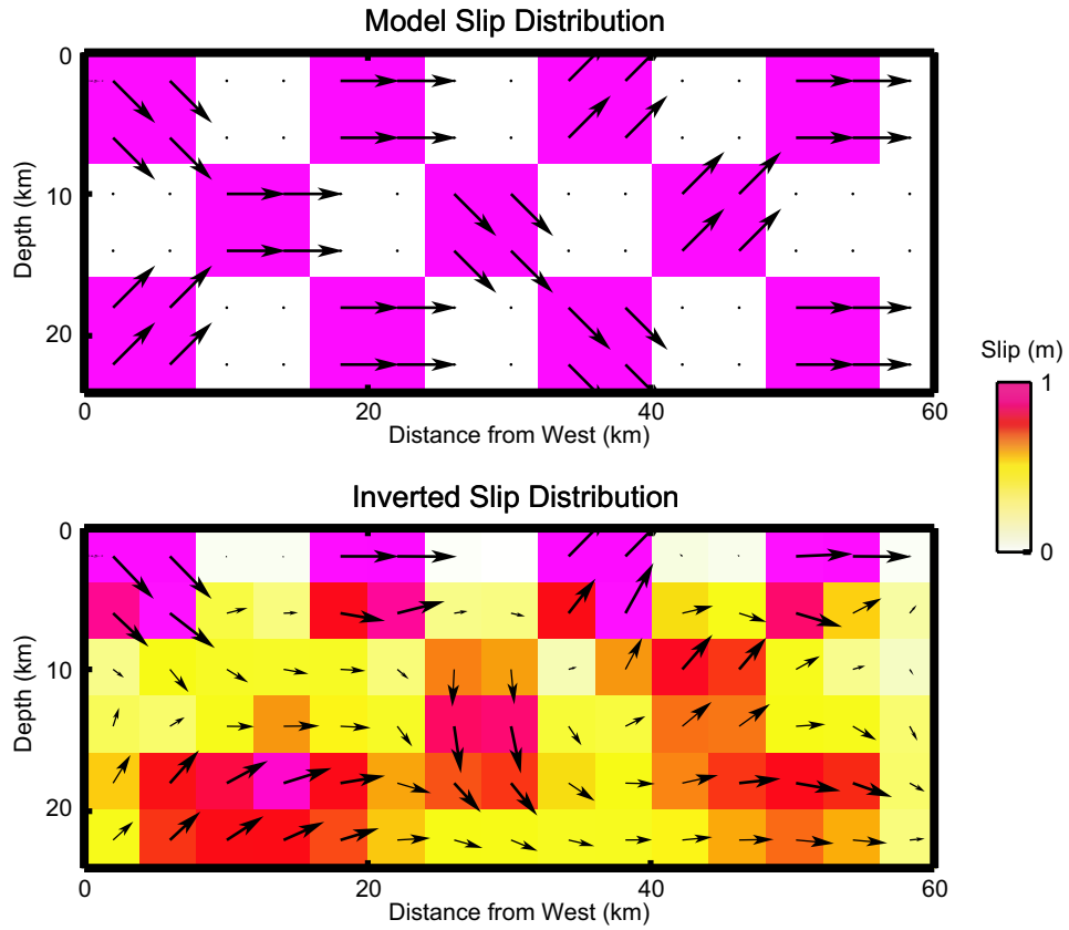
Figure 3. [AUXILLIARY FIGURE 3] Checkerboard resolution test. Phase changes were calculated using the model slip distribution (top), noise was added and and inversion carried out. The smoothing factor was adjusted to find the inverted slip distribution that was closest to the model slip pattern.
