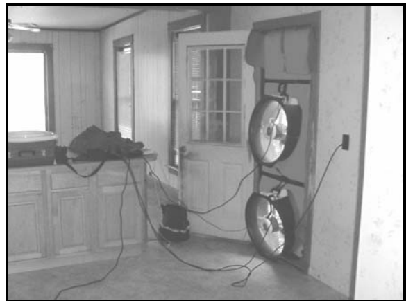
Figure 36: Equipment for Blower Door Test Installed in Door of Vermont House.
