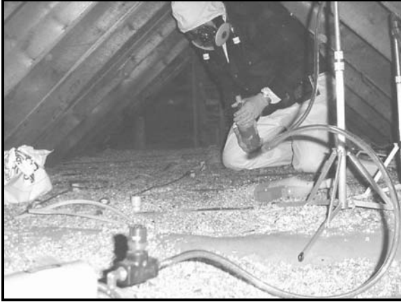
Figure 33: Wet Simulation in Attic of Vermont House - Versar Employee Spraying Water on Attic Insulation During Simulation.
