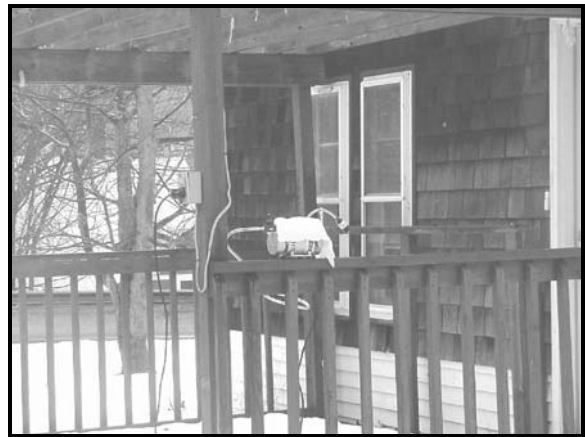
Figure 32: Ambient Air Monitoring Pump and Cassette on Front Porch of Vermont House for Collection of Background Samples
