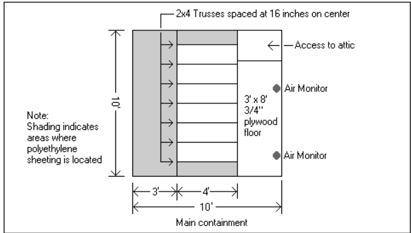
Figure 23 : Top View of Attic Floor (7 feet above main containment floor)
