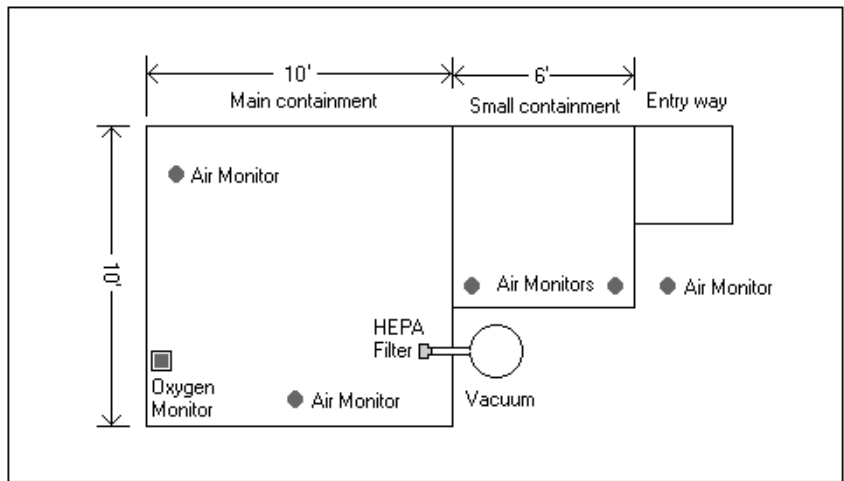
Figure 24 : Top View of Living Space
