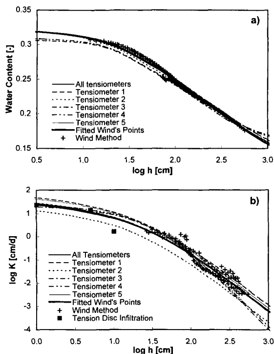
Fig. 5. (a) Water retention curves and (b) hydraulic conductivity functions determined with inverse parameter estimation and Wind's method for Experiment I.
