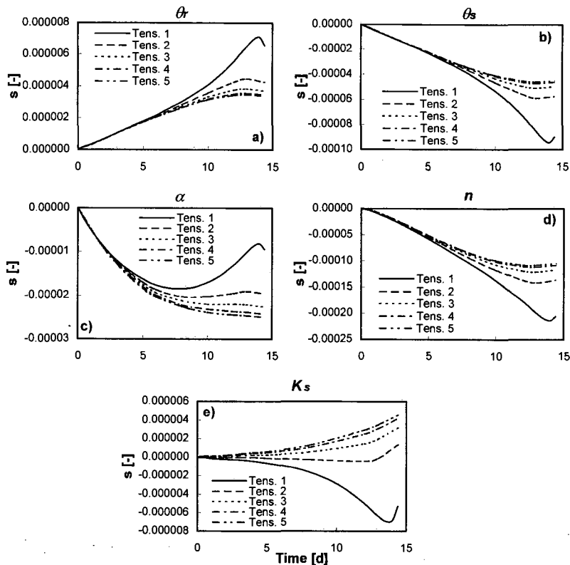
Fig. 3. Sensitivity of the water content \theta to parameters (a) residual soil water content, \theta_r , (b) saturated water content, \theta_s , (c) \alpha , (d) n , and (e) hydraulic conductivity, K_s , as a function of time for a silty soil assuming a one-step evaporation experiment.
