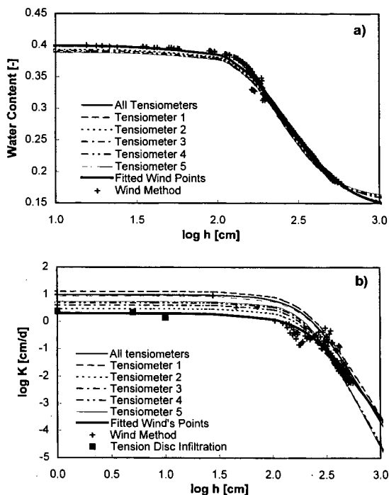
Fig. 7. (a) Water retention curves and (b) hydraulic conductivity functions determined with inverse parameter estimation and Wind's method for Experiment II.
