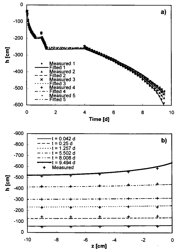
Fig. 8. Measured and fitted tensiometer readings for Experiment II as a function of (a) time and (b) depth.
