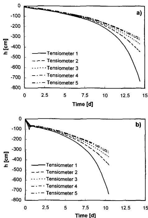
Fig. 1. Simulated pressure heads h for a silty soil for (a) one- and (b) two-step evaporation experiments.
