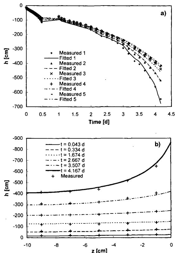
Fig. 6. Measured and fitted tensiometer readings for Experiment I as a function of (a) time and (b) depth.
