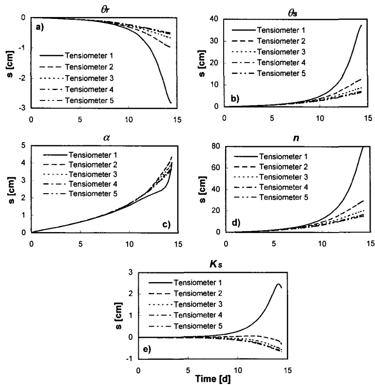
Fig. 2. Sensitivity of the pressure head h to parameters (a) residual soil water content, \theta_r , (b) saturated water content, \theta_s , (c) \alpha , (d) n , and (e) saturated hydraulic conductivity, K_s , as a function of time for a silty soil assuming a one-step evaporation experiment.
