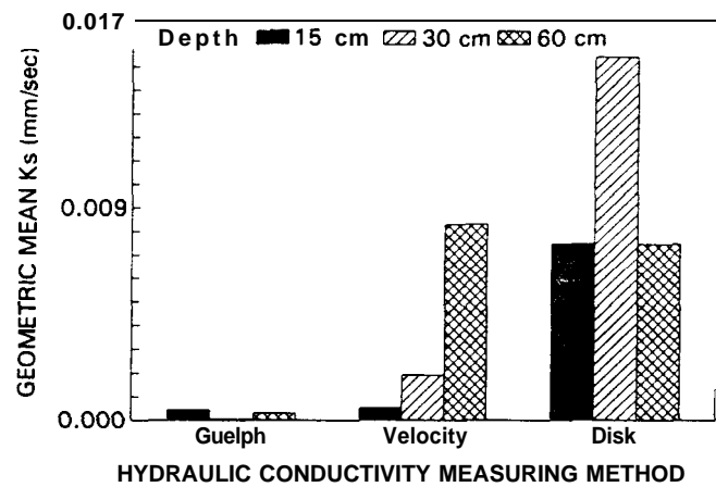
Fig. 3. Comparison of geometric mean saturated hydraulic conductivity ( K_s ) for different methods for individual depths.
