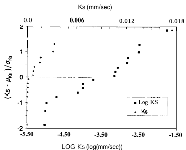
Fig. 1. Fractile diagram of saturated hydraulic conductivity ( K_s ) measured by Guelph permeameter method for raw and log-transformed data.
