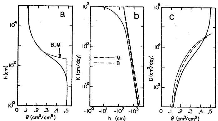
Fig. 4—Comparison of the proposed soil hydraulic functions (solid lines) with curves obtained by applying either the Mualem theory (M; dashed lines) or the Burdine theory (B; dashed-dotted lines) to the Brooks and Corey model of the soil-water retention curve.
