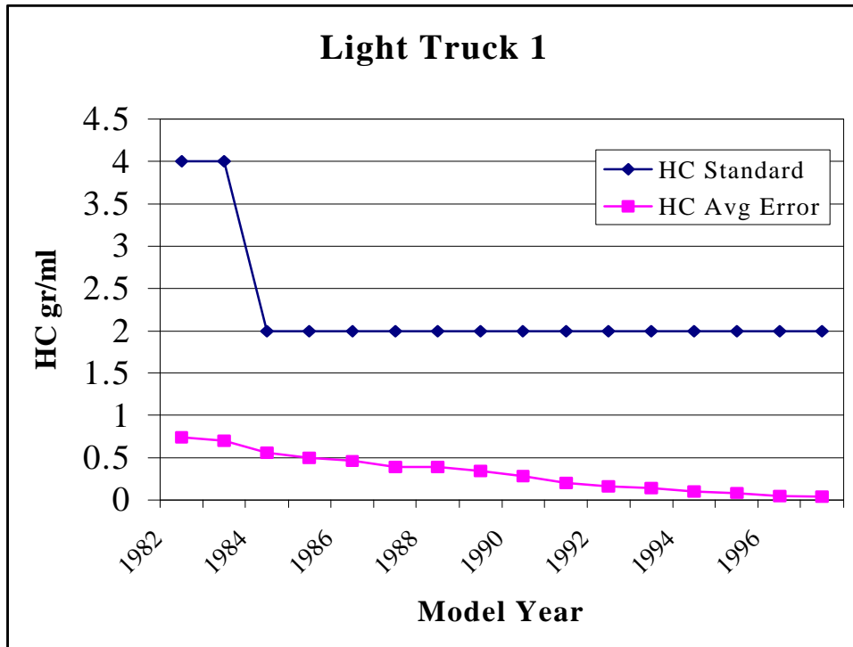
Figure II-2 Light Truck Final High Altitude HC Standards and Projected Fast Pass Result Average Error
