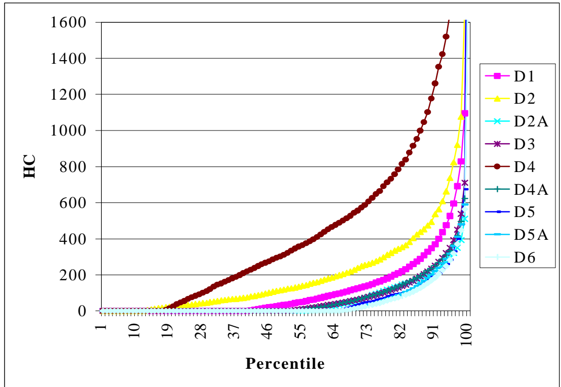
Figure III-12 HC Emissions Distribution by Site
