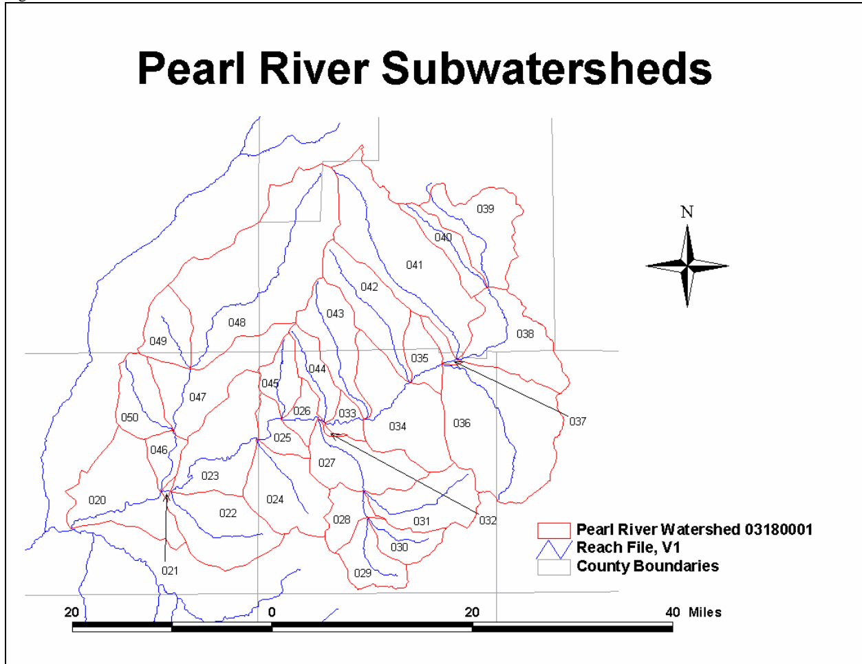
Figure 1.1.2 Pearl River Subwatersheds
