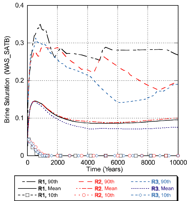
Figure 4-13. Comparison of Brine Saturation in the Waste Panel Between All Replicates, Scenario S1, from the CRA-2004.
