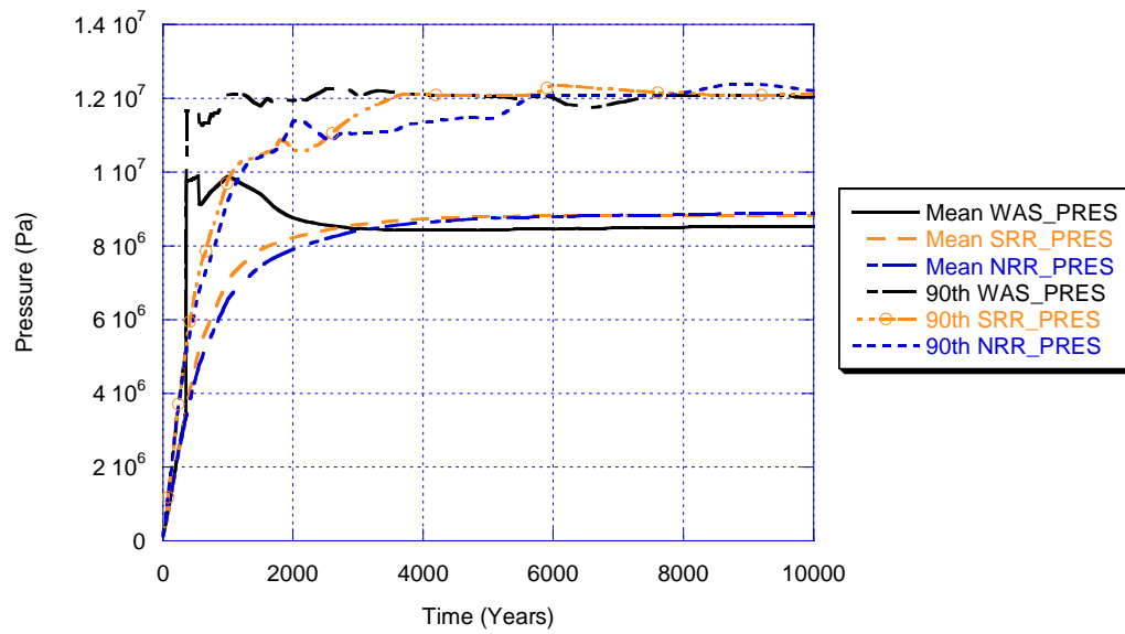
Figure 5-5. Mean And 90 th Percentile Values for Pressure in the Waste Areas Regions of the Repository, Replicate R1, Scenario S2, from the CRA-2004 PABC.
