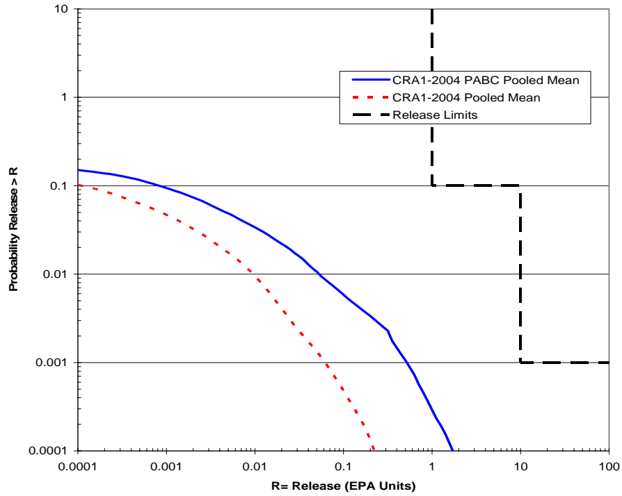
Figure 6-23. Overall Mean CCDFs for DBRs: CRA-2004 PABC and CRA-2004
