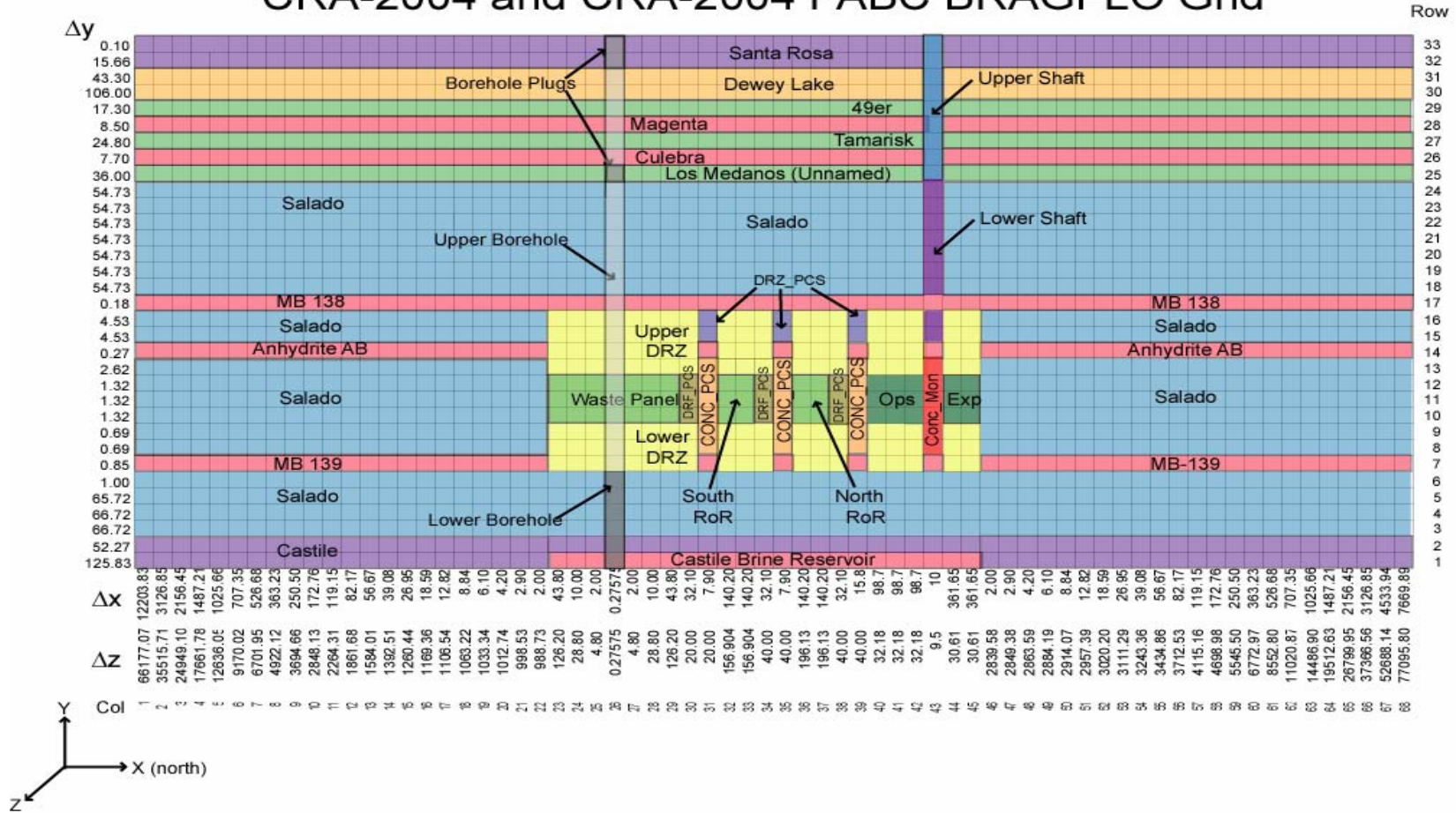
Figure 4-1. CRA-2004 PABC BRAGFLO Grid .
