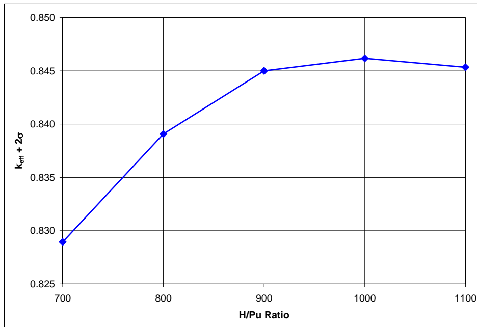
Figure C-, SWB Infinite Storage Array Reactivity as a Function of H/Pu Ratio
