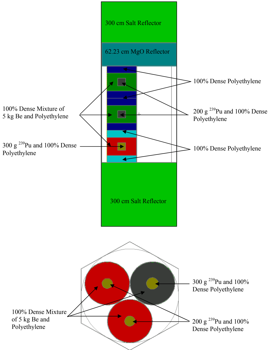
Figure -, Example Array Model for 239 Pu Overbatching in 100-gallon Drum Event
