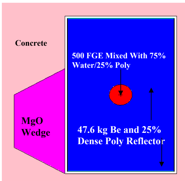
Figure A-, SLB2-SWB Two-container Model
