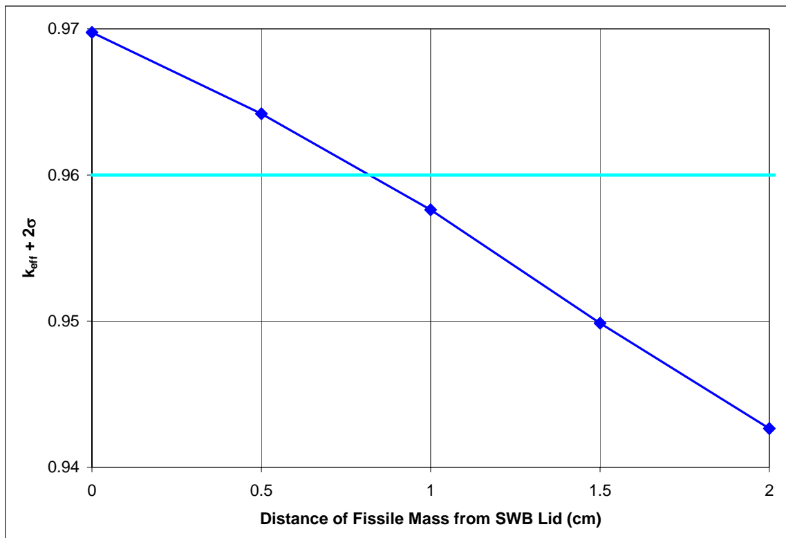
Figure A-, Effect of Separation between Fissile Mass and SWB Lid in Lower SWB in Two-Container Model
