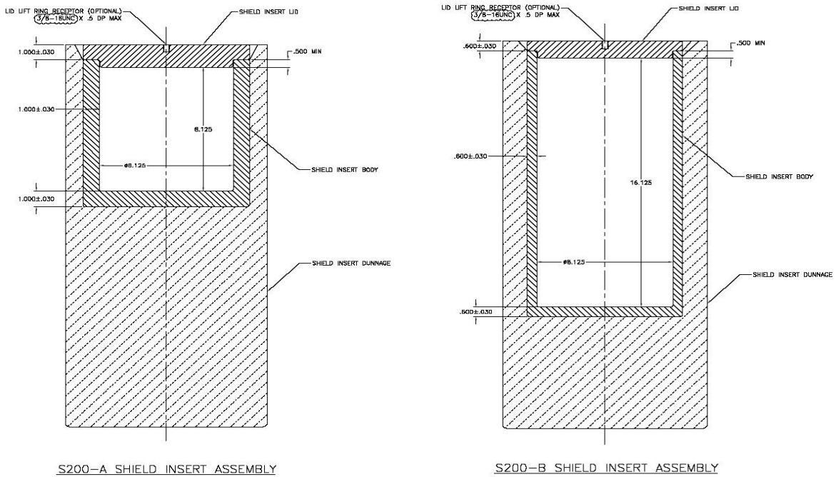
Figure D-, Shielded Insert Options for the S200 12-inch Pipe Components
