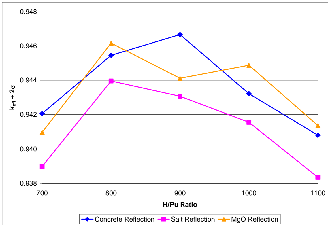
Figure E-, SWB (Direct Loaded Fully Compacted)/55-gallon (100 kg beryllium) Drum Combination
