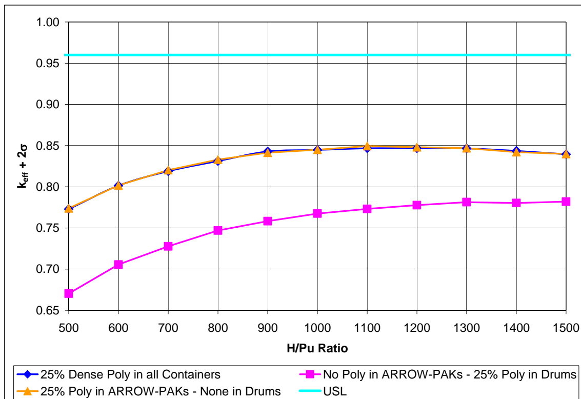
Figure A-1, Underground Array Reactivity for ARROW-PAK™ Containers with Seven-pack of 55-gallon Drums on Top
