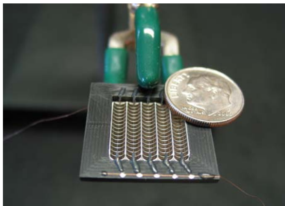
Researchers have developed a new micro-fan only slightly larger than a dime. The new fan can generate winds on the same scale as a laptop computer fan, but uses far less energy. Credit: Dan Schlitz and Vishal Singhal, Thorn Micro Technologies
