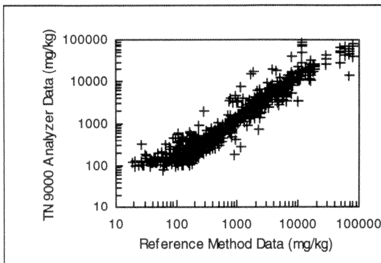
Figure 5-2. Critical Zone for the Determination of a Field-based Method Detection Limit for Copper: Between 100 and 200 mg/kg for the reference data, the linear relationship between the two data sets changes. This point of change identified the point at which field-based MDLs for the analyzer were determined.
