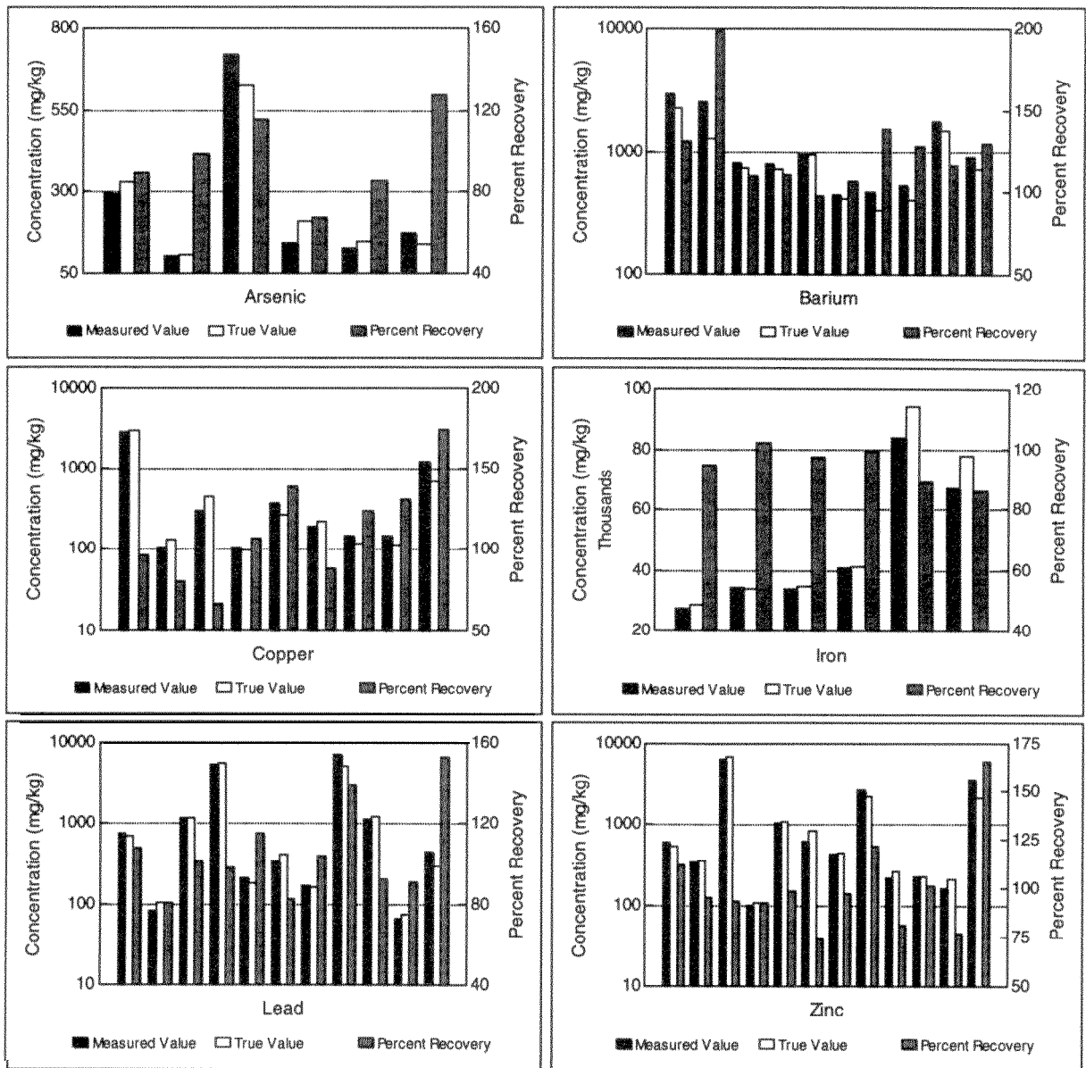
Figure 5-6. SRM Results—TN 9000 Analyzer: These graphs illustrate the relationship between the analyzer’s data (measured values) and the true values for the SRMs. The gray bars represent the percent recovery for the analyzer. Each set of three bars (black, white, and gray) represents a single SRM sample.
