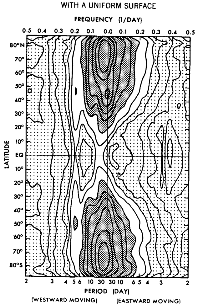
FIG. 3. Latitude–frequency distribution (wavenumber 1) of the space–time power spectral density ( m^2 \text{ day} ) of geopotential height at 515 mb over three year's data of the model with a uniform surface. Dark shade indicates greater than 500, light shade less than 100. Contour intervals 10, 20, 50, 100, 200, 500, 1000, 2000, 5000, 10000. These values should be divided by 365 to be consistent with the units in Fig. 2.
