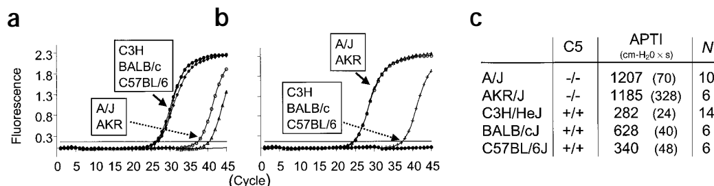
Figure 2. C5 allele correlates with allergen-induced AHR across inbred strains. A/J have a 5' deletion in the C5 gene and carry the C5-D allele; C3H/HeJ mice do not have the deletion and carry the C5-S allele. Allele-specific kinetic polyacrylamide gel electrophoresis (PCR) was used to genotype other inbred mouse strains. (a) Kinetic PCR using the C3H/HeJ allele-specific primer identifies the C5-S allele in three strains. Primer dimer formation is detected in strains
