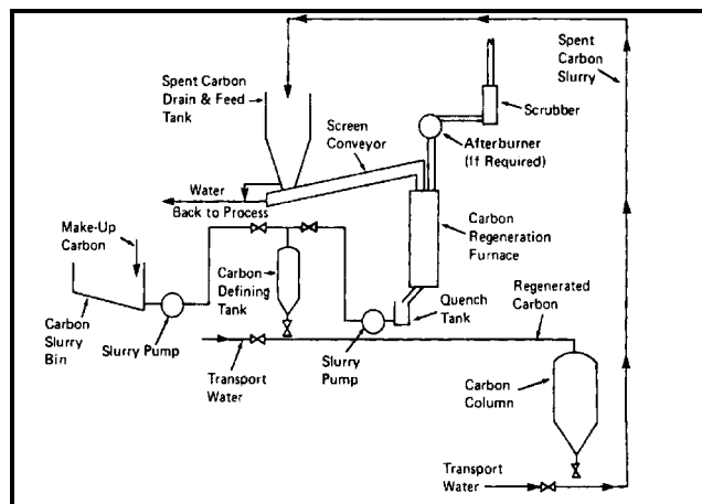
FIGURE 1 GAC ADSORPTION SCHEMATIC
