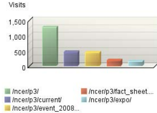
Single-Page Visits
