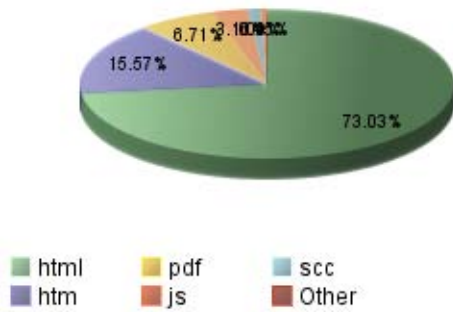
Uploaded Files
