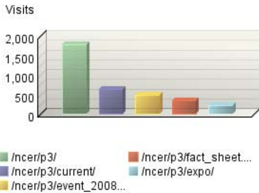
Exit Pages
