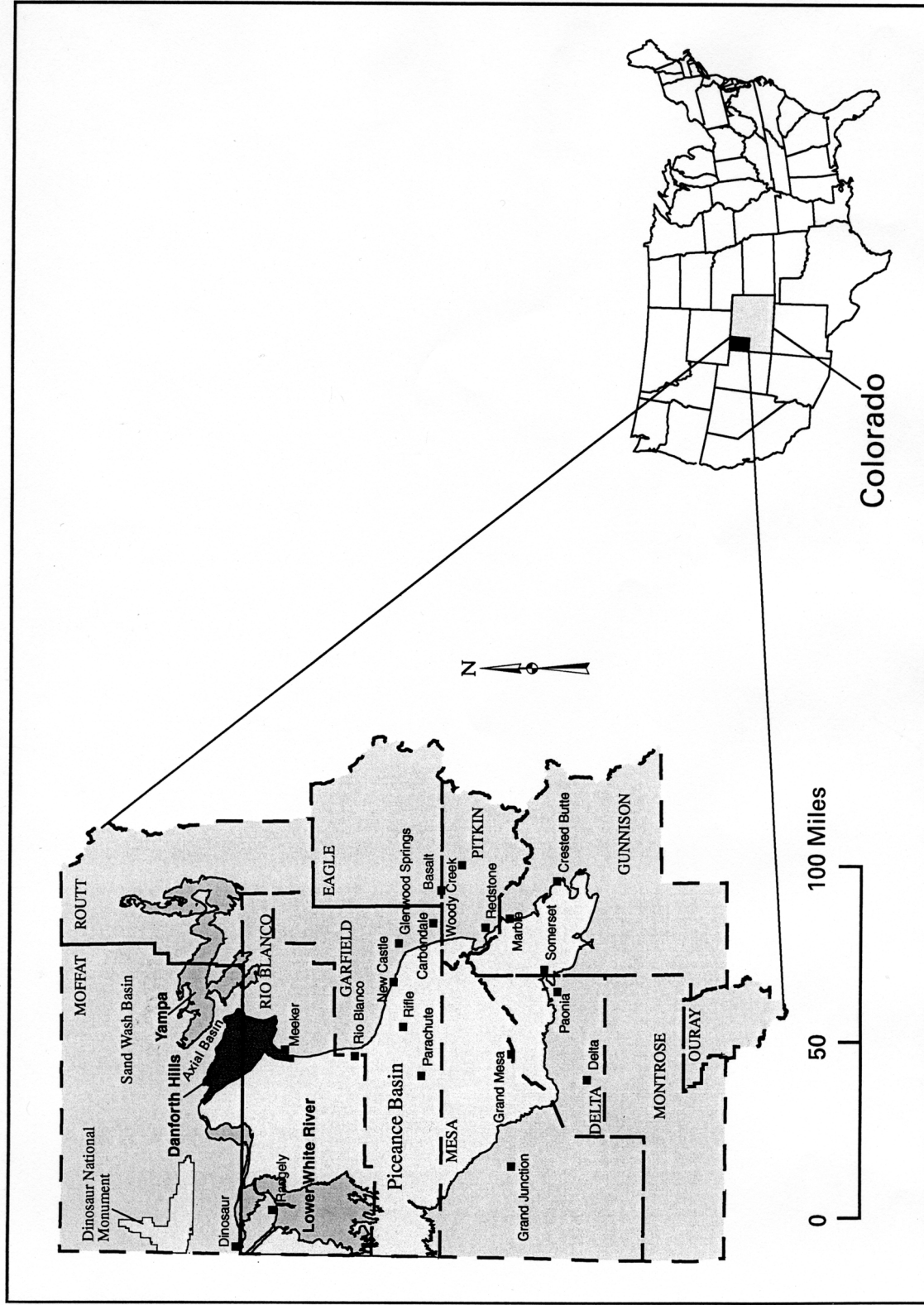
Figure 3-17. Coal Fields in Moffat, Rio Blanco and Routt Counties, Colorado
