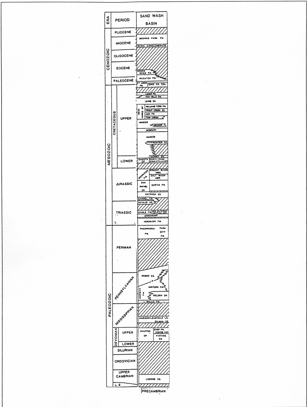
Figure 3-14. Geologic Stratigraphic Columnar Section
