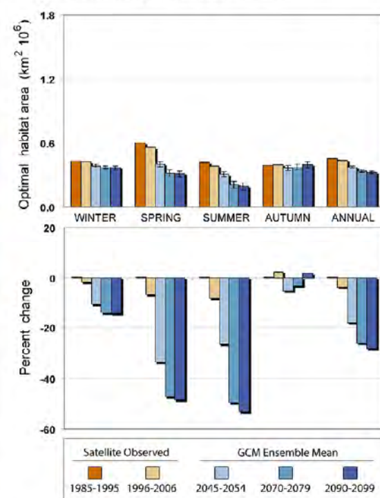
c) Canada-Greenland
