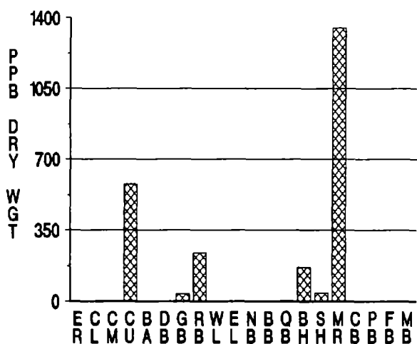
PERYLENE
