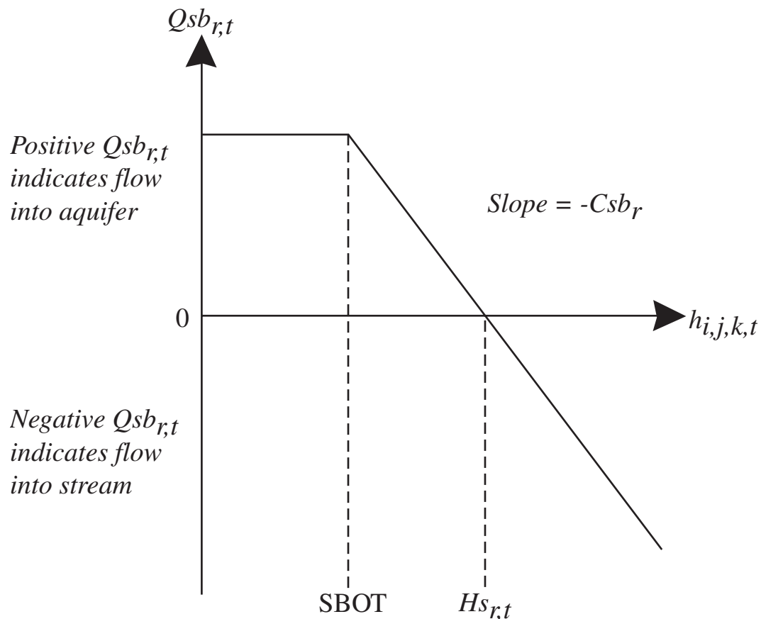
Figure 1. Seepage rate, Q_{sb,r,t} , through a streambed as a function of ground-water head, h_{i,j,k,t} , in a model cell, where SBOT is the streambed bottom, C_{sb_r} is streambed conductance, and H_{s,r,t} is head in the stream. Figure modified from Prudic (1989).
