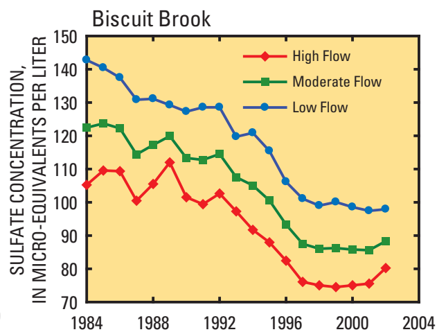
Figure 4. Trends in sulfate concentrations during high flow, moderate flow, and low flow conditions for the Biscuit Brook watershed in the Catskill Mountains in southeastern N.Y. High flow shows as upturn in sulfate concentrations during the last 2 years of record that is not apparent at low flow.
