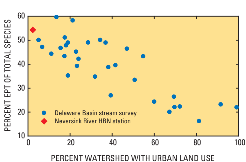
Figure 3. Effect of urbanization on stream macroinvertebrate populations in streams of the Delaware River Basin. EPT (Ephemeroptera, Plecoptera, and Trichoptera) richness is an index of river health based on the populations of mayfly, stonefly, and caddisfly, respectively (modified from Fischer and others, 2004).
