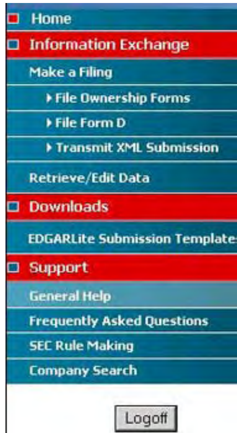
Figure 9-4: EDGAR Menu
