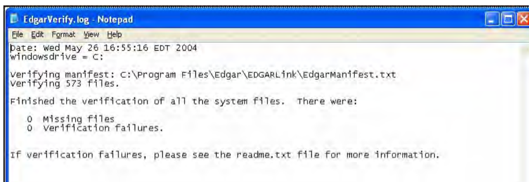
Figure 7-11: EdgarVerify.log Report
