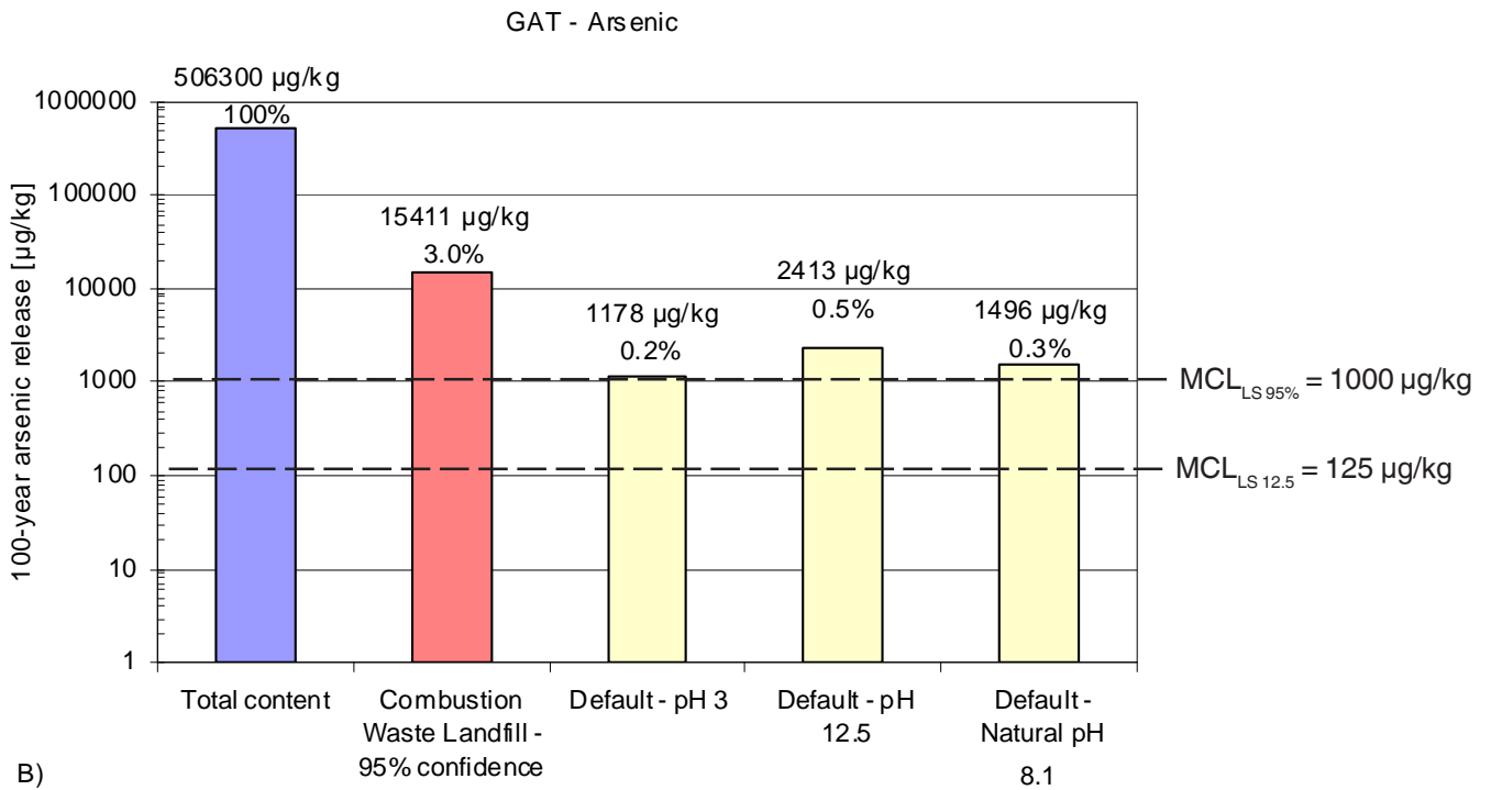
Figure G-13. 100-Year Arsenic Release Estimates from A) Baseline Fly Ash and B) Fly Ash with ACI. Release estimates for percolation controlled scenario are compared to release estimate based on total content. The amount of the arsenic that would be released if the release concentration was at the MCL is also shown for comparison (LS default scenario = 12.5 L/kg and LS 95% = 100 L/kg).
