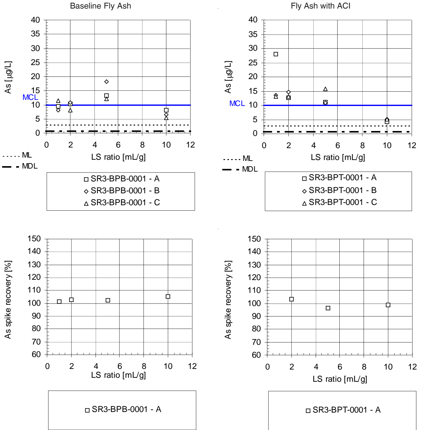
Figure D-6. Arsenic Release (top) and Spike Recoveries (bottom) as a Function of LS Ratio for the Baseline Fly Ash and the Fly Ash with Enhanced Hg Control.
