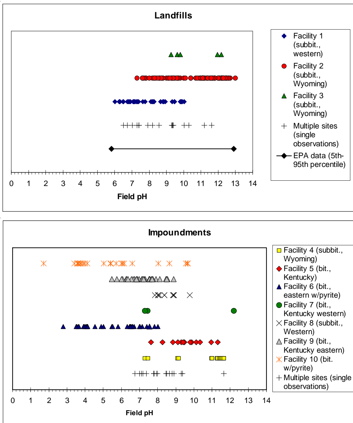
Figure 14. Range of pH Observed in Field Leachate at Landfills and Impoundments Used for Disposal of CCRs—from EPRI Database. Also included is the range (5 th –95 th percentile) of pH values for CCR landfills reported in the EPA database (EPA, 2000). Facilities 6 and 10 have co-disposal of pyrite from mill rejects with CCRs. Data does not include facilities with scrubbers. Primary data from EPRI (EPRI, 2005).
