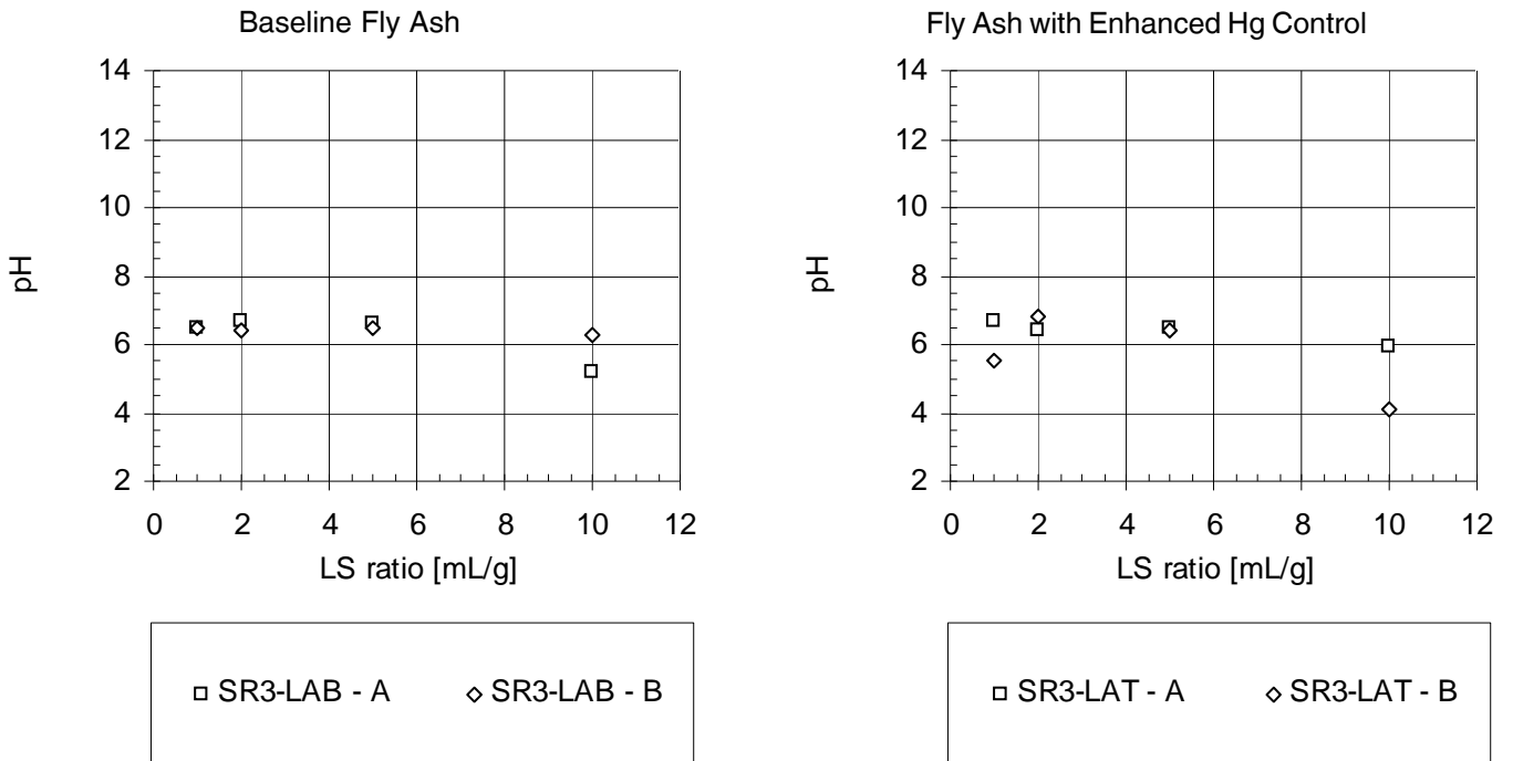
Figure I-2. pH as a Function of LS Ratio for the Baseline Fly Ash and the Fly Ash with Enhanced Hg Control.
