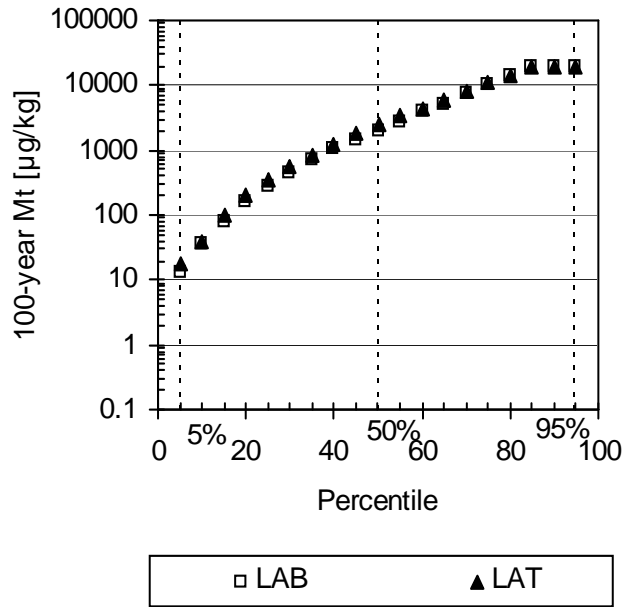
Figure I-11. 100-Year Arsenic Release Estimates as a Function of the Cumulative Probability for the Scenario of Disposal in a Combustion Waste Landfill.
