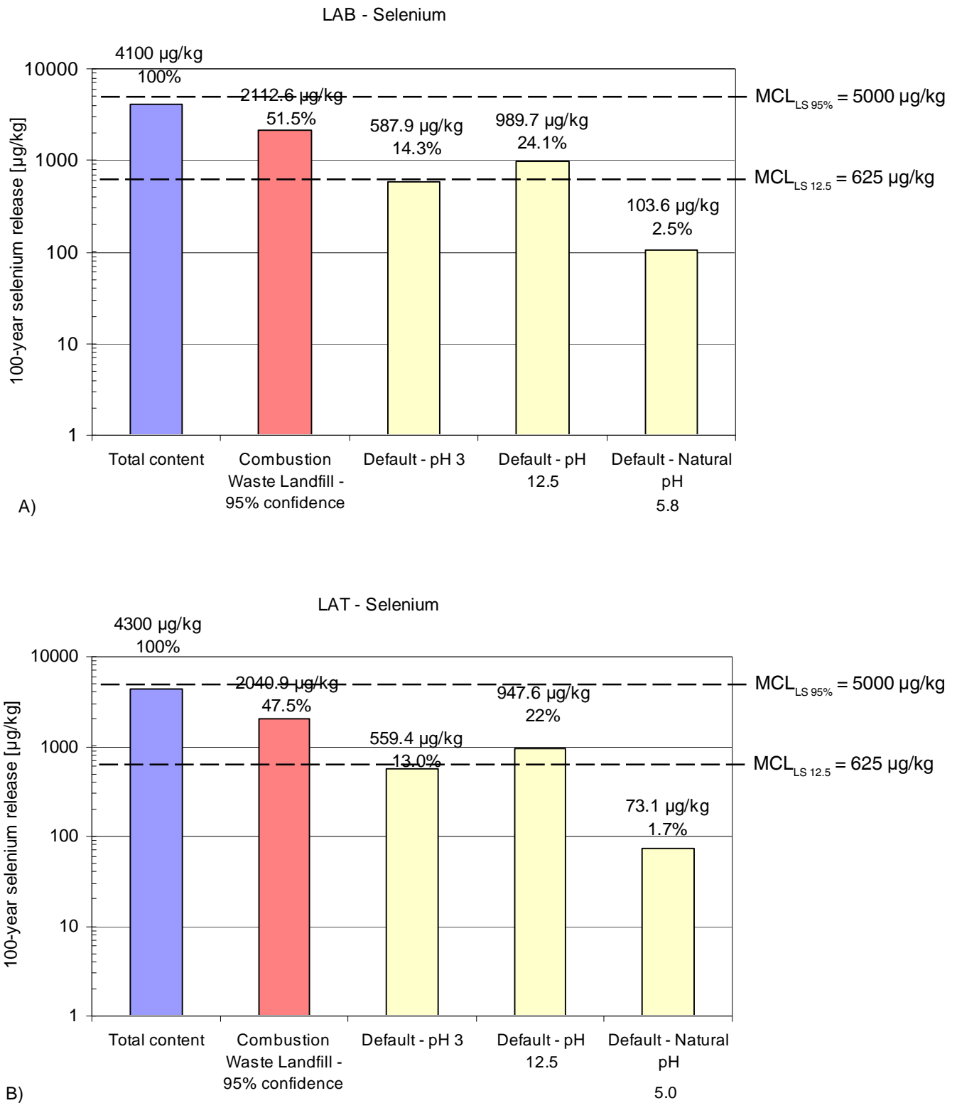
Figure I-14. 100-year Selenium Release Estimates from A) Baseline Fly Ash and B) Fly Ash with Enhanced Hg Control. Release estimates for percolation controlled scenario are compared to release estimate based on total content. The amount of the selenium that would be released if the release concentration was at the MCL is also shown for comparison (LS default scenario = 12.5 L/kg and LS 95% = 100 L/kg).
