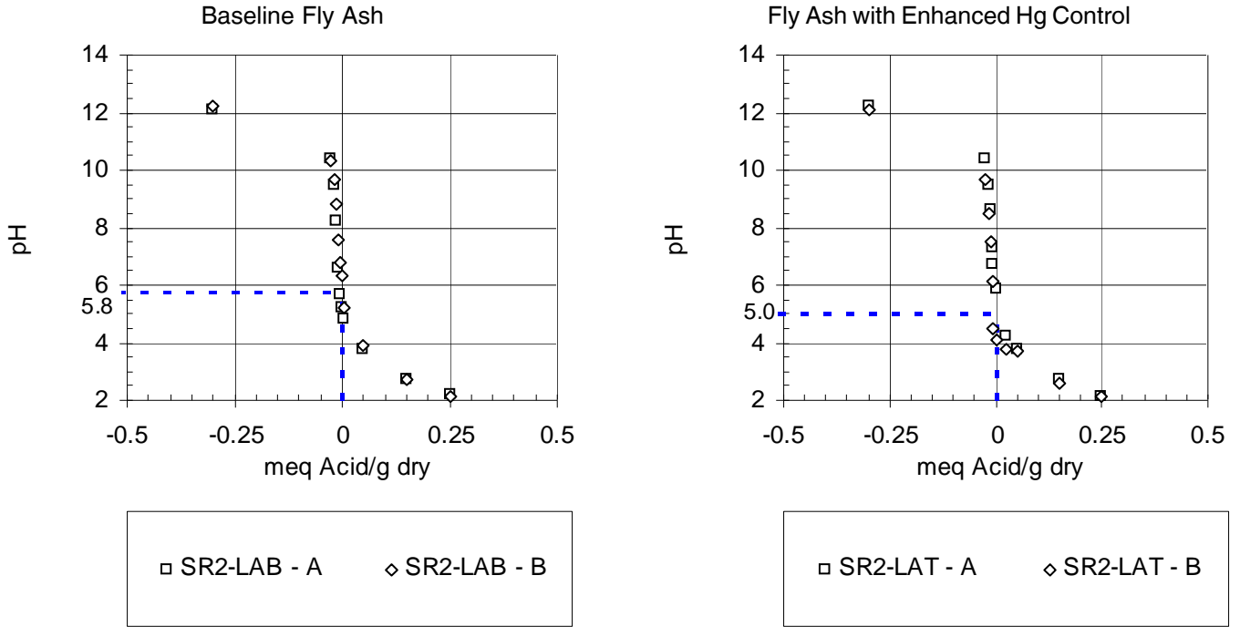
Figure I-1. pH Titration Curves for the Baseline Fly Ash and the Fly Ash with Enhanced Hg Control.
