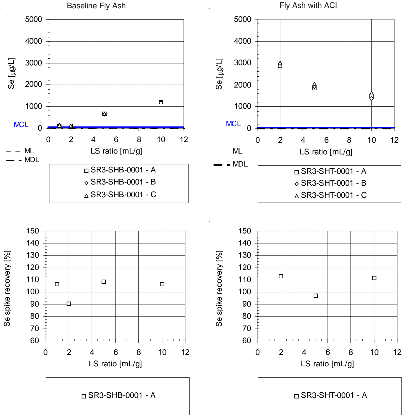
Figure F-8. Selenium Release (top) and Spike Recoveries (bottom) as a Function of LS Ratio for the Baseline Fly Ash and the Fly Ash with Enhanced Hg Control.
