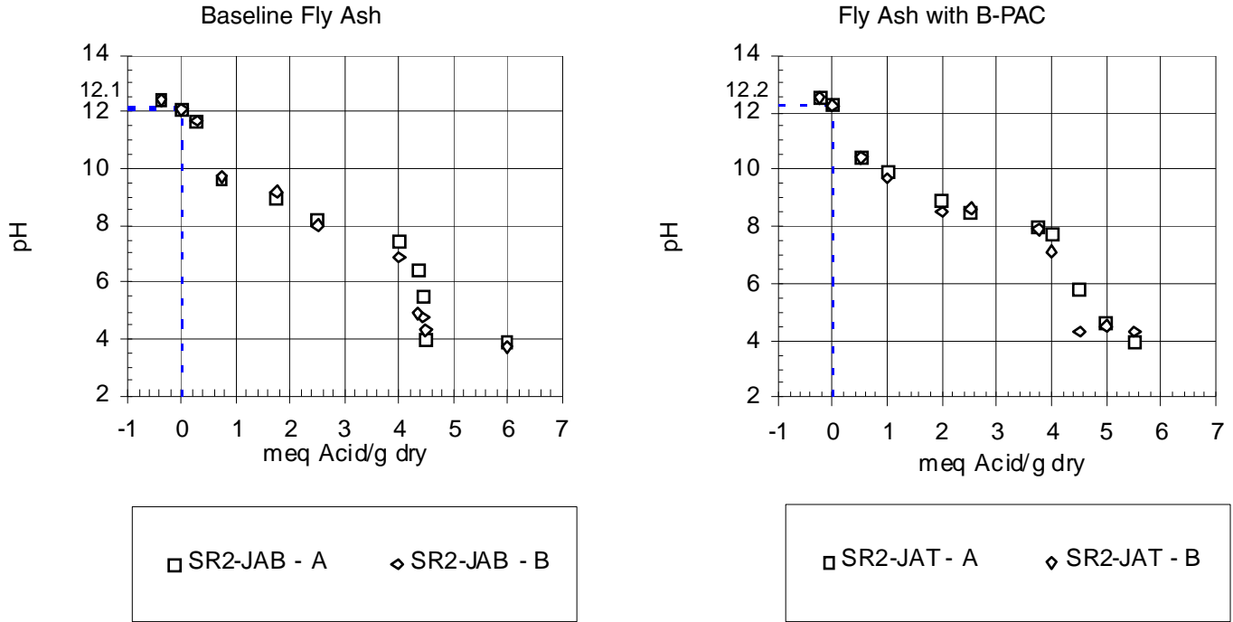
Figure H-1. pH Titration Curves for the Baseline Fly Ash and the Fly Ash with Enhanced Hg Control.
