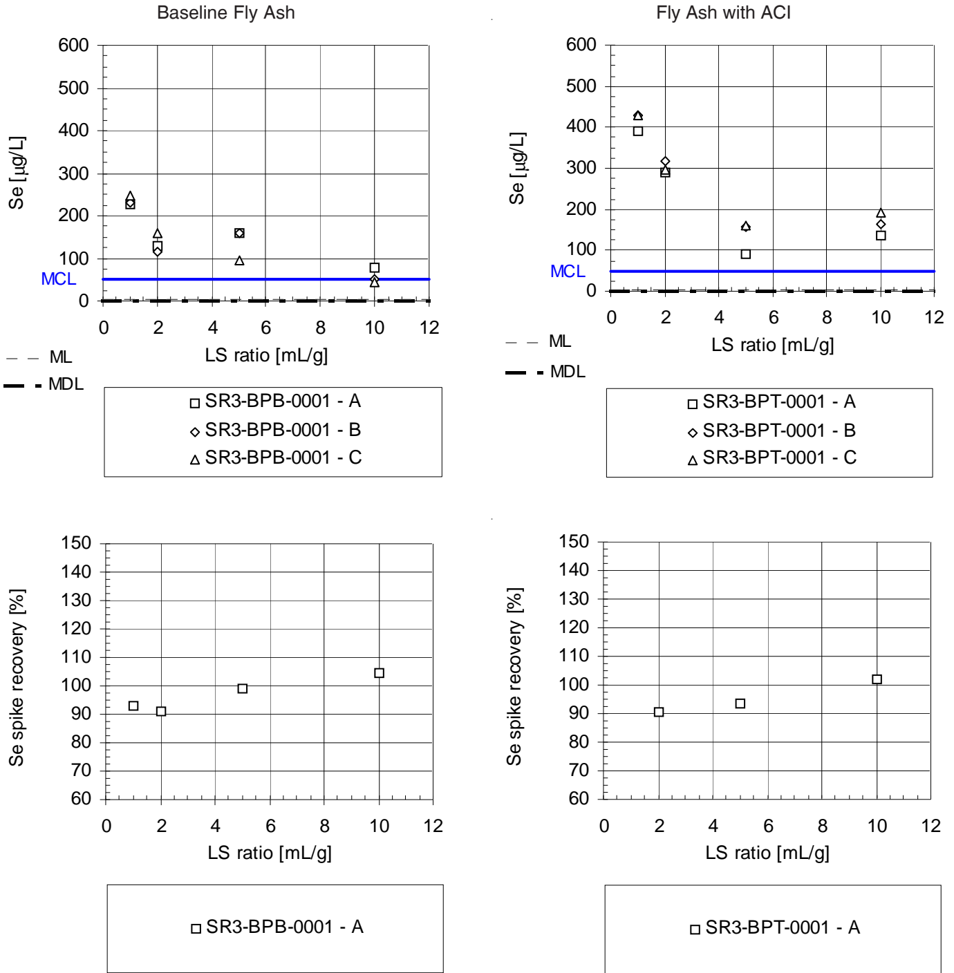
Figure D-8. Selenium Release (top) and Spike Recoveries (bottom) as a Function of LS Ratio for the Baseline Fly Ash and the Fly Ash with Enhanced Hg Control.
