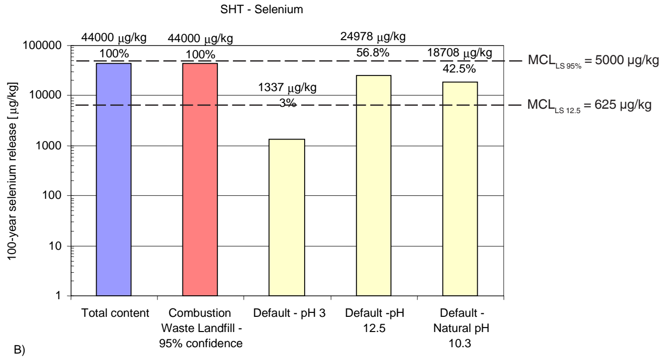
Figure F-14. 100-year Selenium Release Estimates from A) Baseline Fly Ash and B) Fly Ash with ACI. Release estimates for percolation controlled scenario are compared to release estimate based on total content. The amount of the selenium that would be released if the release concentration was at the MCL is also shown for comparison ( LS_{\text{default scenario}} = 12.5 \text{ L/kg} and LS_{95\%} = 100 \text{ L/kg} ).
