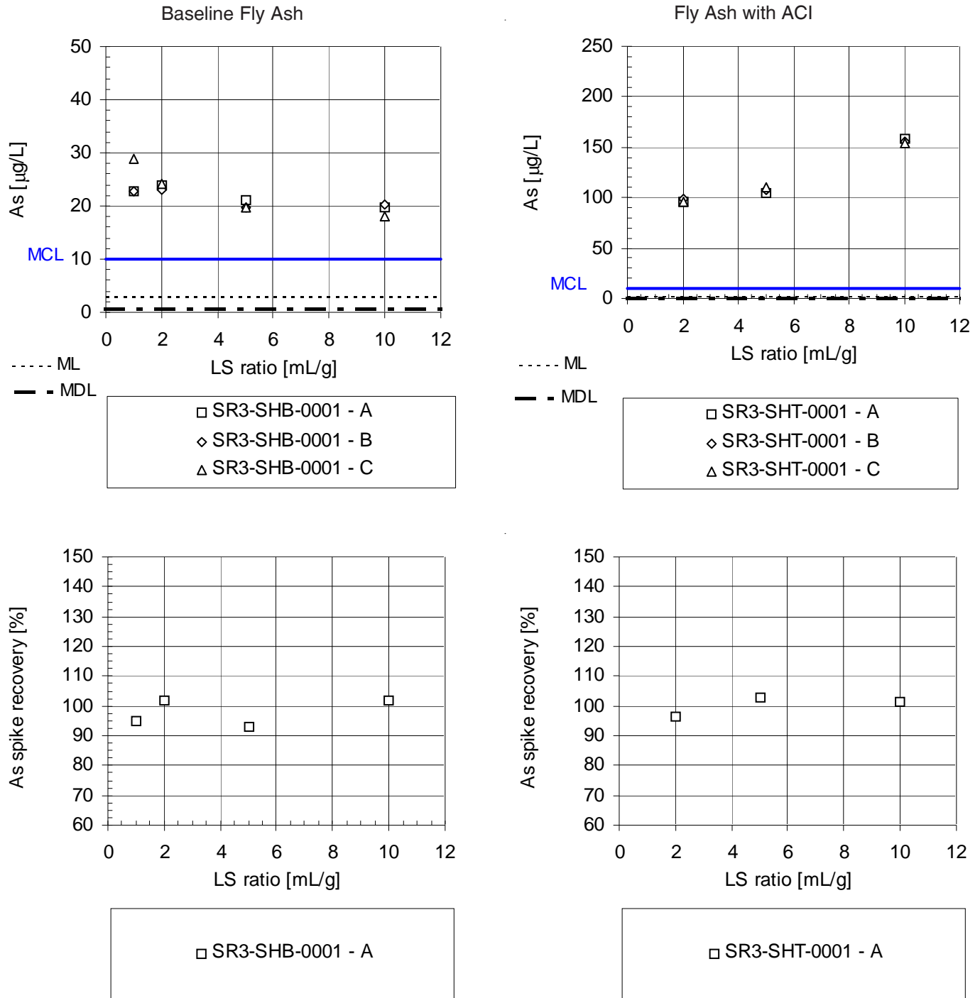
Figure F-6. Arsenic Release (top) and Spike Recoveries (bottom) as a Function of LS Ratio for the Baseline Fly Ash and the Fly Ash with Enhanced Hg Control.
