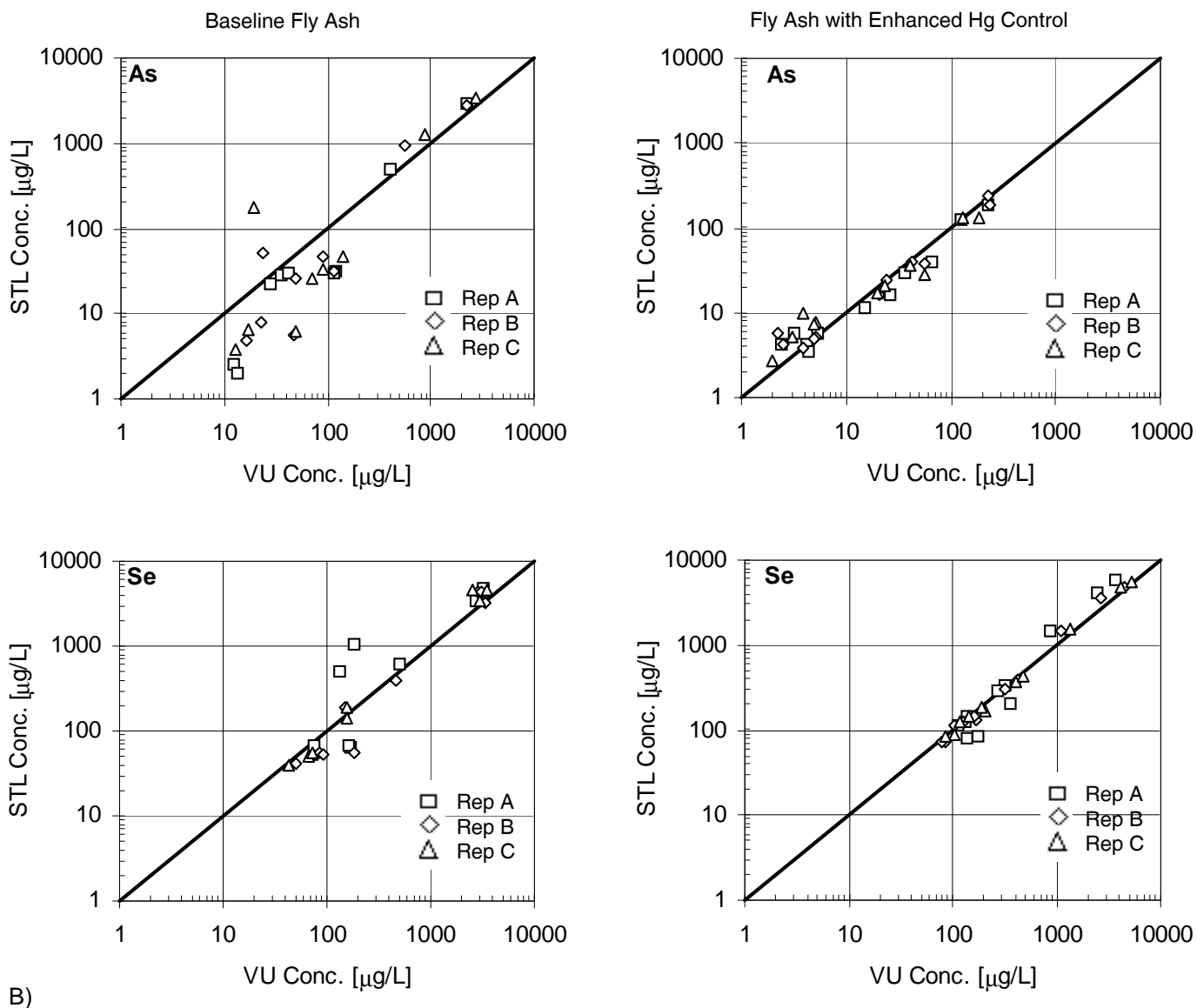
Figure 17. STL Versus Vanderbilt Analytical Results for Arsenic and Selenium from Sr002.1. Baseline Fly Ash and Fly Ash with Enhanced Hg Control from Brayton Point Are Shown.
