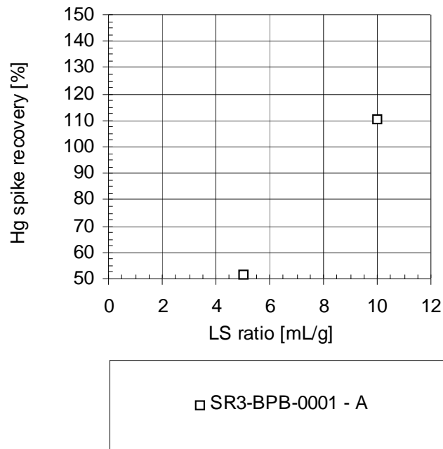
Figure D-4. Mercury Release (top) and Spike Recoveries (bottom) as a Function of LS Ratio for the Baseline Fly Ash and the Fly Ash with Enhanced Hg Control.
