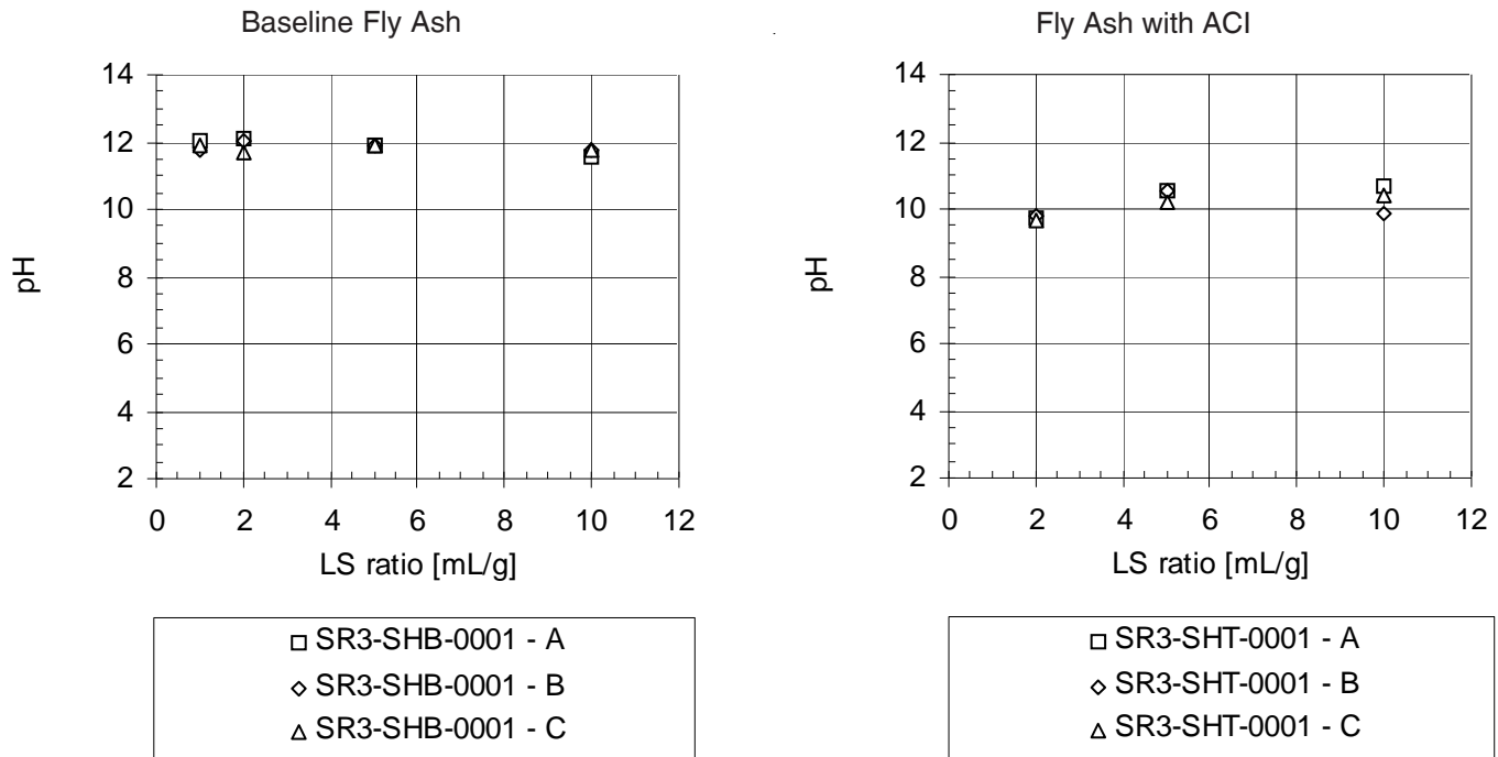
Figure F-2. pH as a Function of LS Ratio for the Baseline Fly Ash and the Fly Ash with Enhanced Hg Control.
