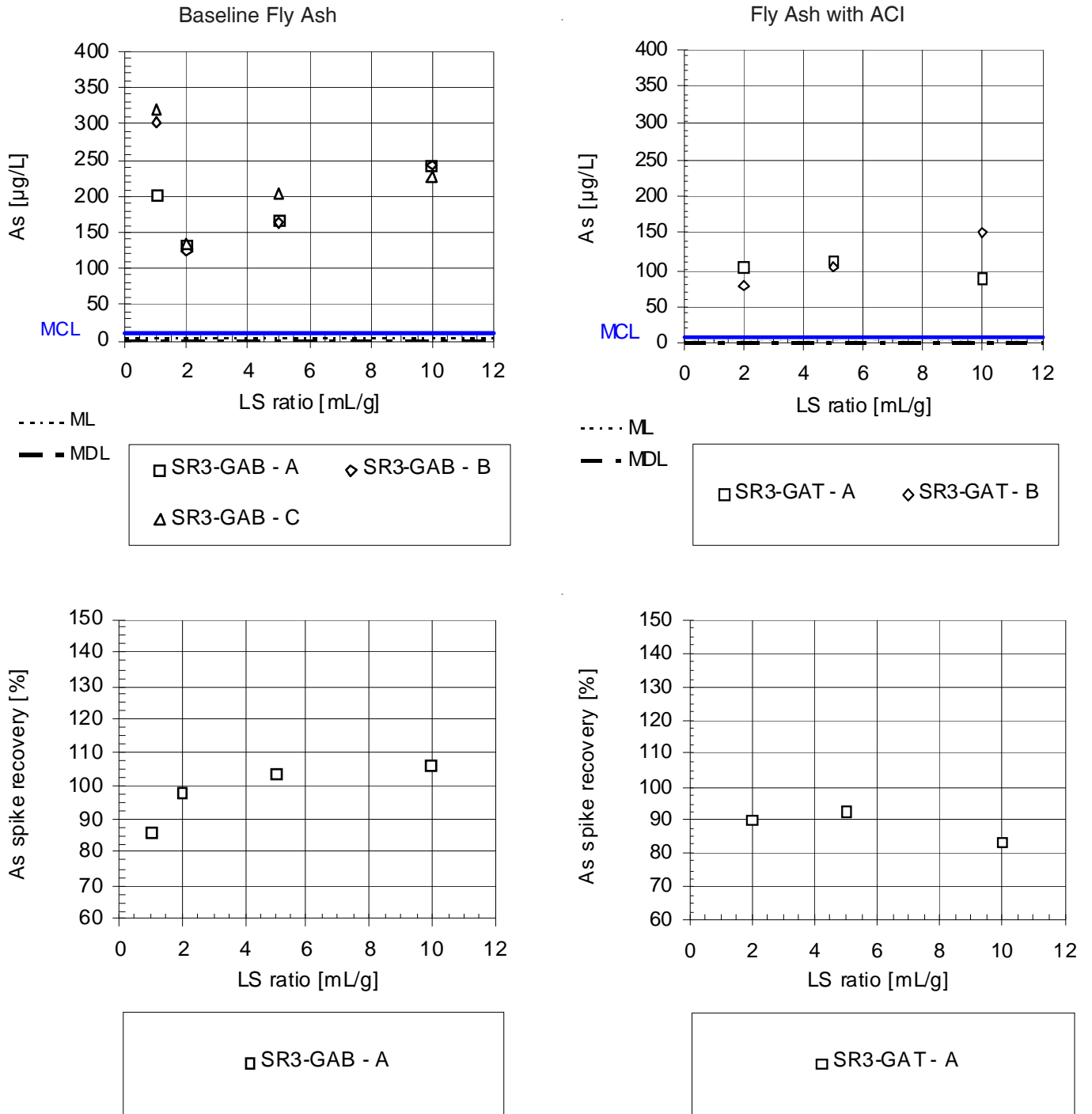
Figure G-6. Arsenic Release (top) and Spike Recoveries (bottom) as a Function of LS Ratio for the Baseline Fly Ash and the Fly Ash with Enhanced Hg Control.
