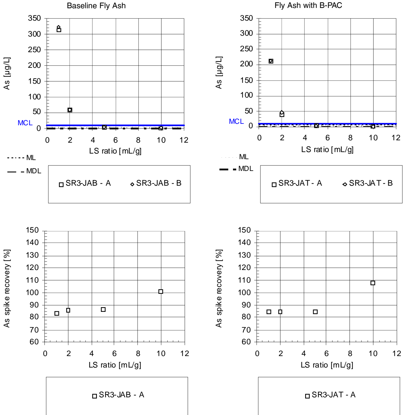
Figure H-6. Arsenic Release (top) and Spike Recoveries (bottom) as a Function of LS Ratio for the Baseline Fly Ash and the Fly Ash with Enhanced Hg Control.
