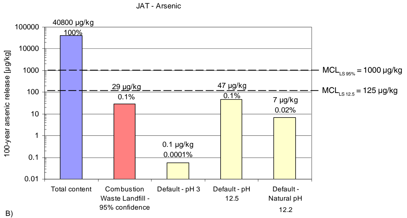
Figure H-13. 100-Year Arsenic Release Estimates from A) Baseline Fly Ash and B) Fly Ash with B-PAC. Release estimates for percolation controlled scenario are compared to release estimate based on total content. The amount of the arsenic that would be released if the release concentration was at the MCL is also shown for comparison ( LS_{\text{default scenario}} = 12.5 \text{ L/kg} and LS_{95\%} = 100 \text{ L/kg} ).
