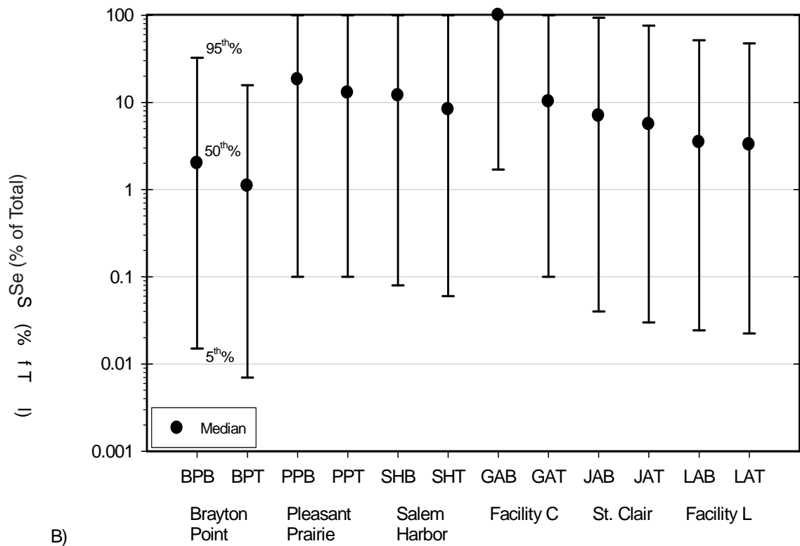
Figure 30. Upper Bound of 100 yr Selenium Release Estimates for Landfill Scenario Without and with Activated Carbon Injection. (A) mass released in \mu\text{g} of selenium released per kg of CCR and total content in \mu\text{g} of selenium per kg of CCR, (B) percent of total selenium content released. Symbol with error bars represents 5 th , 50 th and 95 th percentiles from Monte Carlo simulation. (Facility code suffixes B = baseline and T = treated with sorbent injection; for example, PPB = Pleasant Prairie baseline, and PPT = Pleasant Prairie treated)
