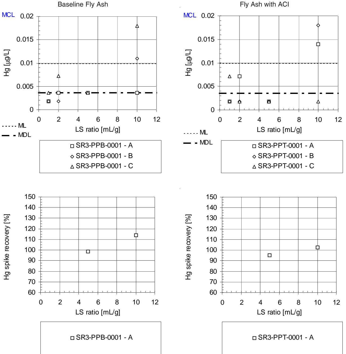
Figure E-4. Mercury Release (top) and Spike Recoveries (bottom) as a Function of LS Ratio for the Baseline Fly Ash and the Fly Ash with Enhanced Hg Control.
