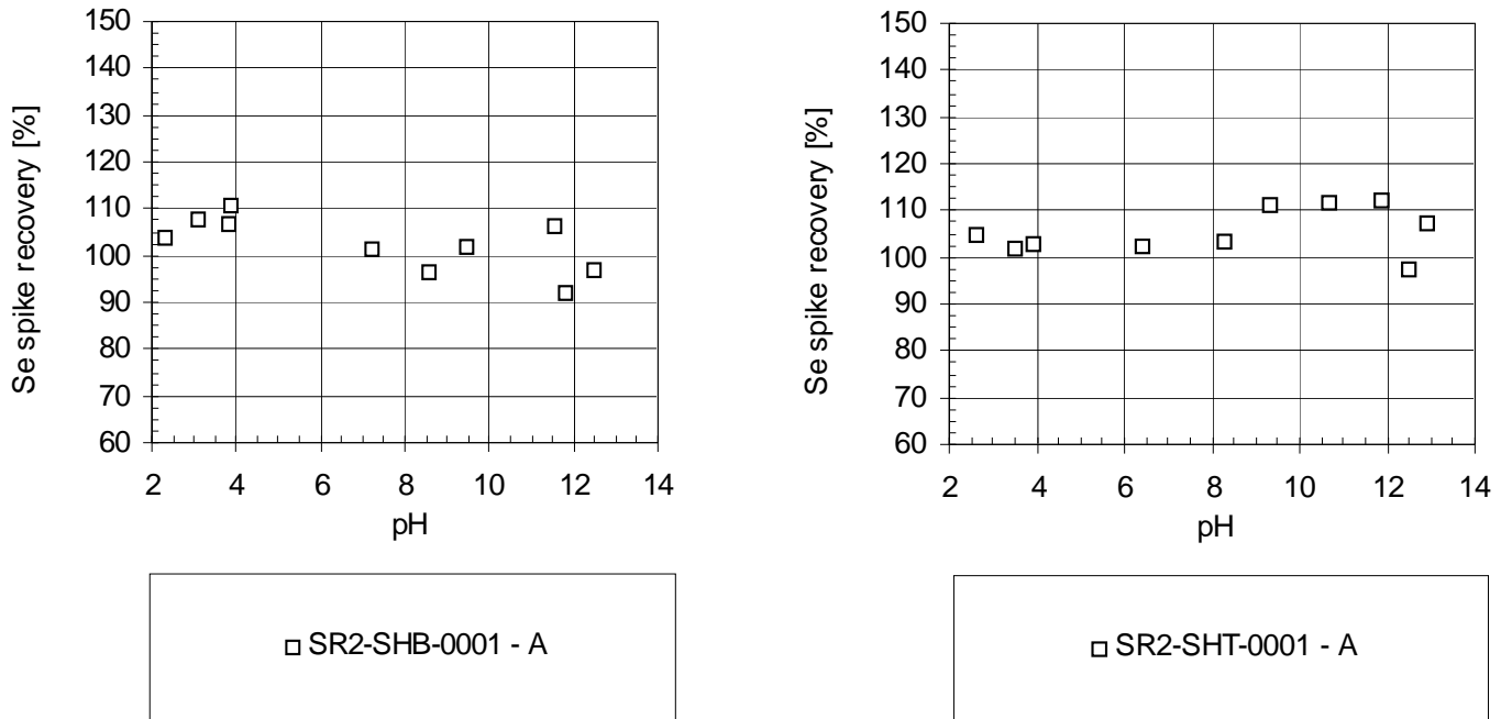
Figure F-7. Selenium Release (top) and Spike Recoveries (bottom) as a Function of pH for the Baseline Fly Ash and the Fly Ash with Enhanced Hg Control. 5 th and 95 th percentiles of selenium concentrations observed in typical combustion waste landfill leachate are shown for comparison.
