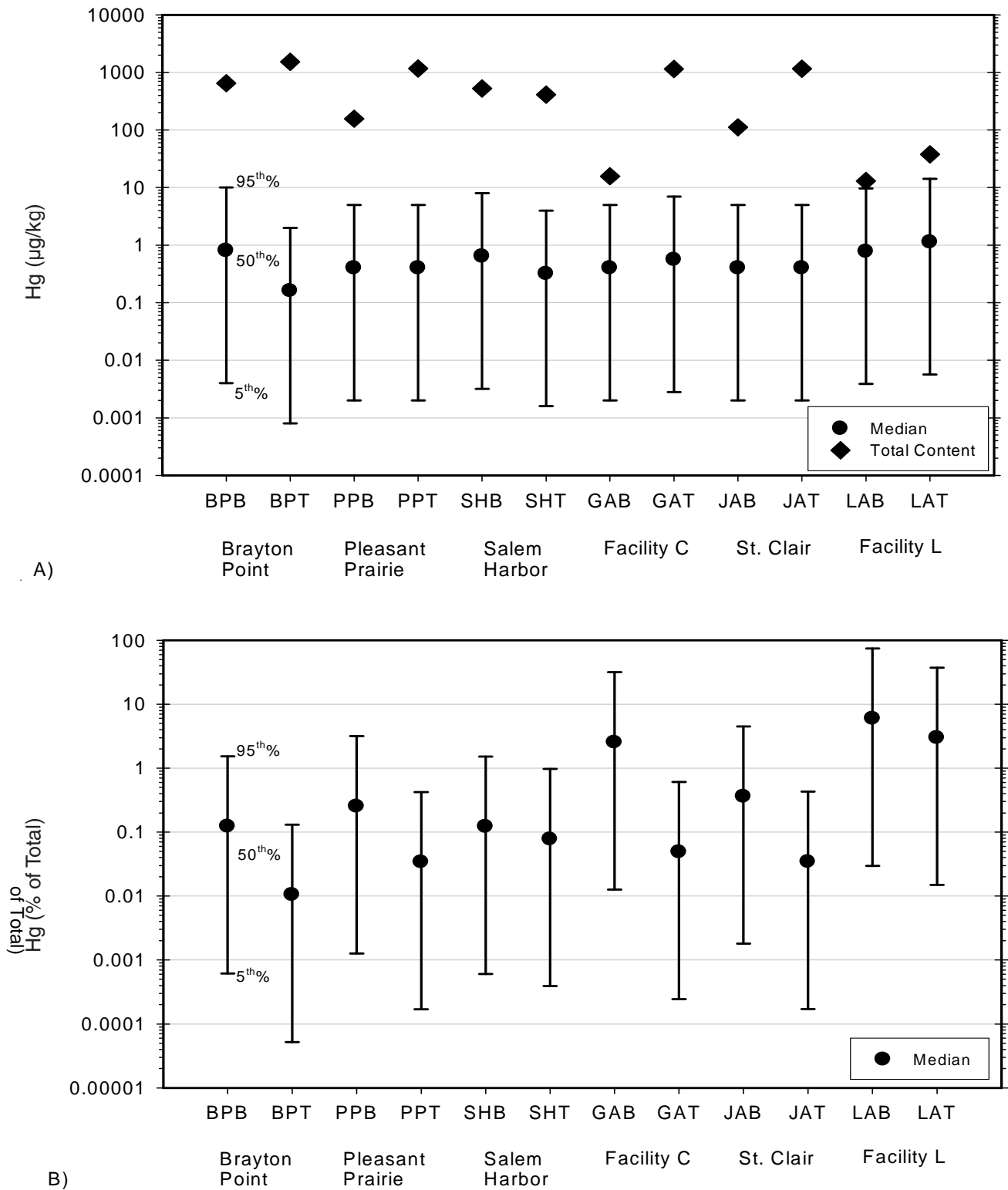
Figure 28. Upper Bound of 100 yr Mercury Release Estimates for Landfill Scenario Without and with Activated Carbon Injection. (A) mass released in µg of mercury released per kg of CCR and total content in µg of mercury per kg of CCR, (B) percent of total mercury content released. Symbol with error bars represents 5 th , 50 th and 95 th percentiles from Monte Carlo simulation. (Facility code suffixes B = baseline and T = treated with sorbent injection; for example, PPB = Pleasant Prairie baseline, and PPT = Pleasant Prairie treated)
