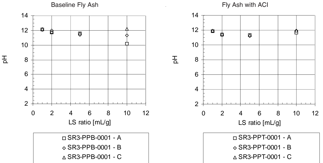
Figure E-2. pH as a Function of LS Ratio for the Baseline Fly Ash and the Fly Ash with Enhanced Hg Control.
