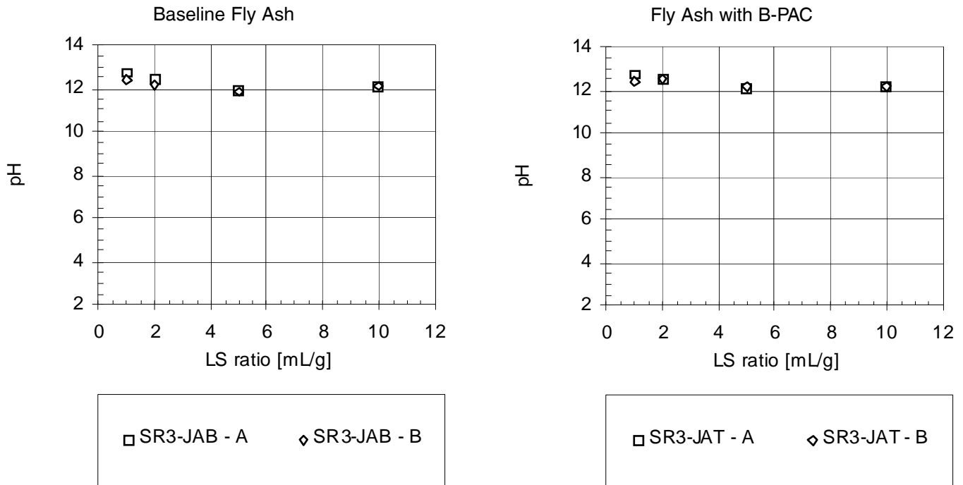
Figure H-2. pH as a Function of LS Ratio for the Baseline Fly Ash and the Fly Ash with Enhanced Hg Control.
