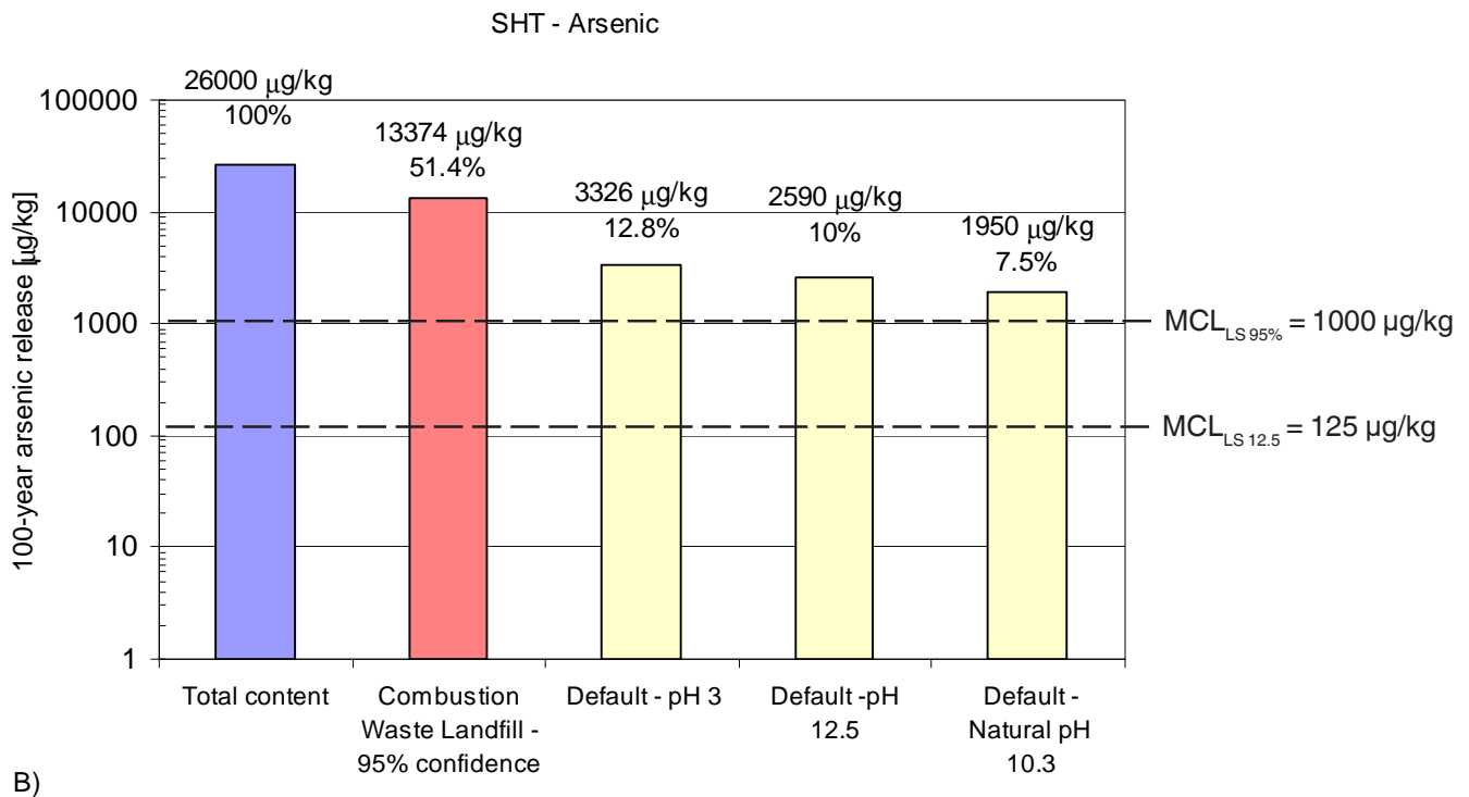
Figure F-13. 100-Year Arsenic Release Estimates from A) Baseline Fly Ash and B) Fly Ash with ACI. Release estimates for percolation controlled scenario are compared to release estimate based on total content. The amount of the arsenic that would be released if the release concentration was at the MCL is also shown for comparison ( LS_{\text{default scenario}} = 12.5 \text{ L/kg} and LS_{95\%} = 100 \text{ L/kg} ).
