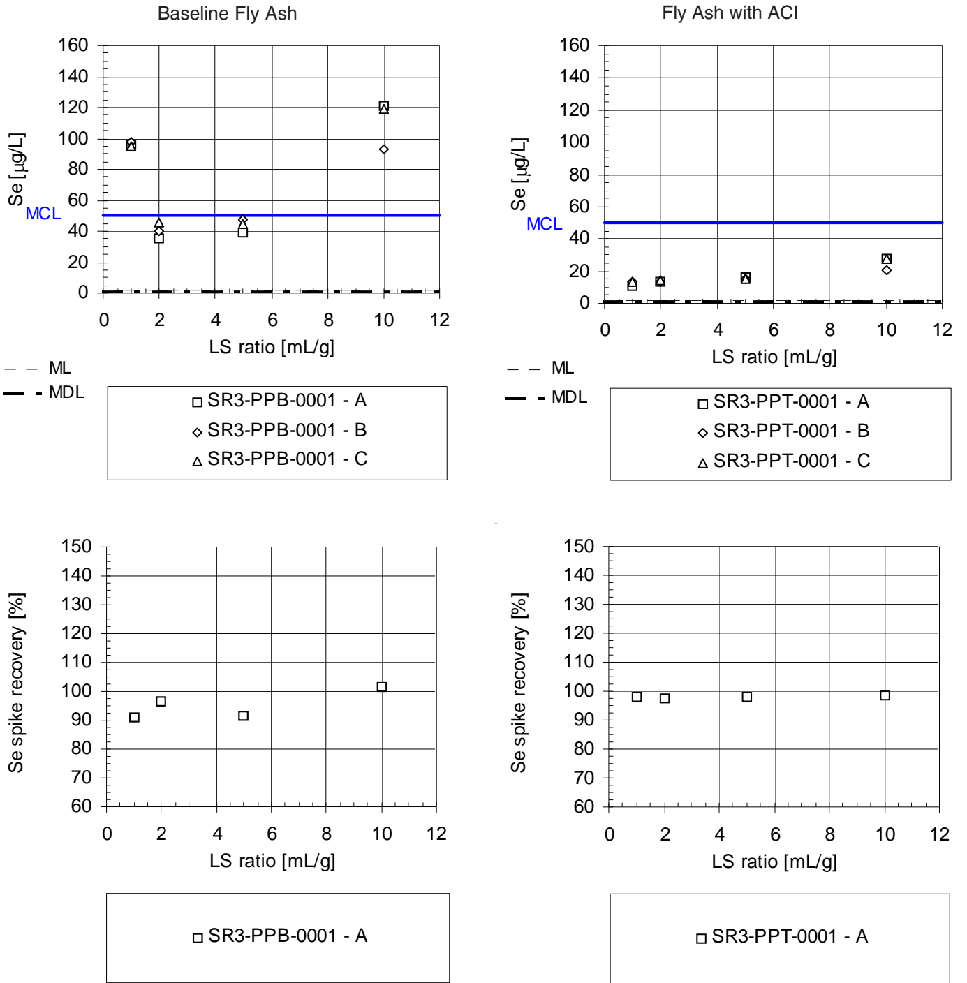
Figure E-8. Selenium Release (top) and Spike Recoveries (bottom) as a Function of LS Ratio for the Baseline Fly Ash and the Fly Ash with Enhanced Hg Control.
