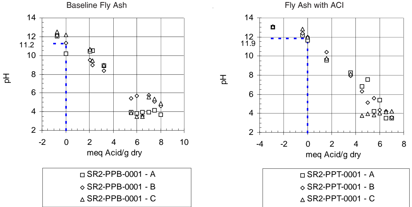
Figure E-1. pH Titration Curves for the Baseline Fly Ash and the Fly Ash with Enhanced Hg Control.
