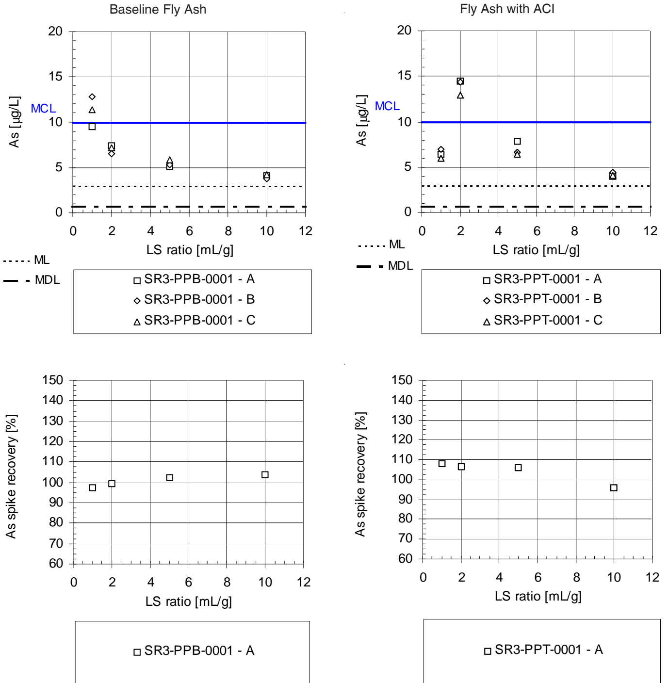
Figure E-6. Arsenic Release (top) and Spike Recoveries (bottom) as a Function of LS Ratio for the Baseline Fly Ash and the Fly Ash with Enhanced Hg Control.
