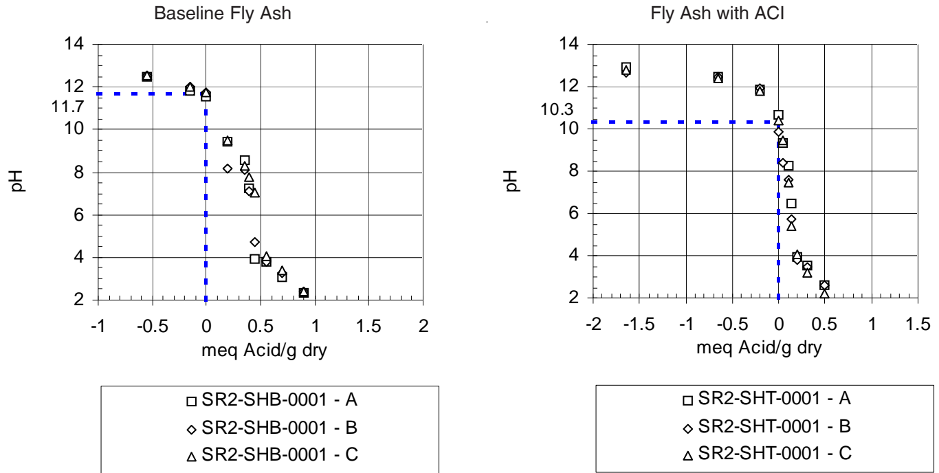
Figure F-1. pH Titration Curves for the Baseline Fly Ash and the Fly Ash with Enhanced Hg Control.
