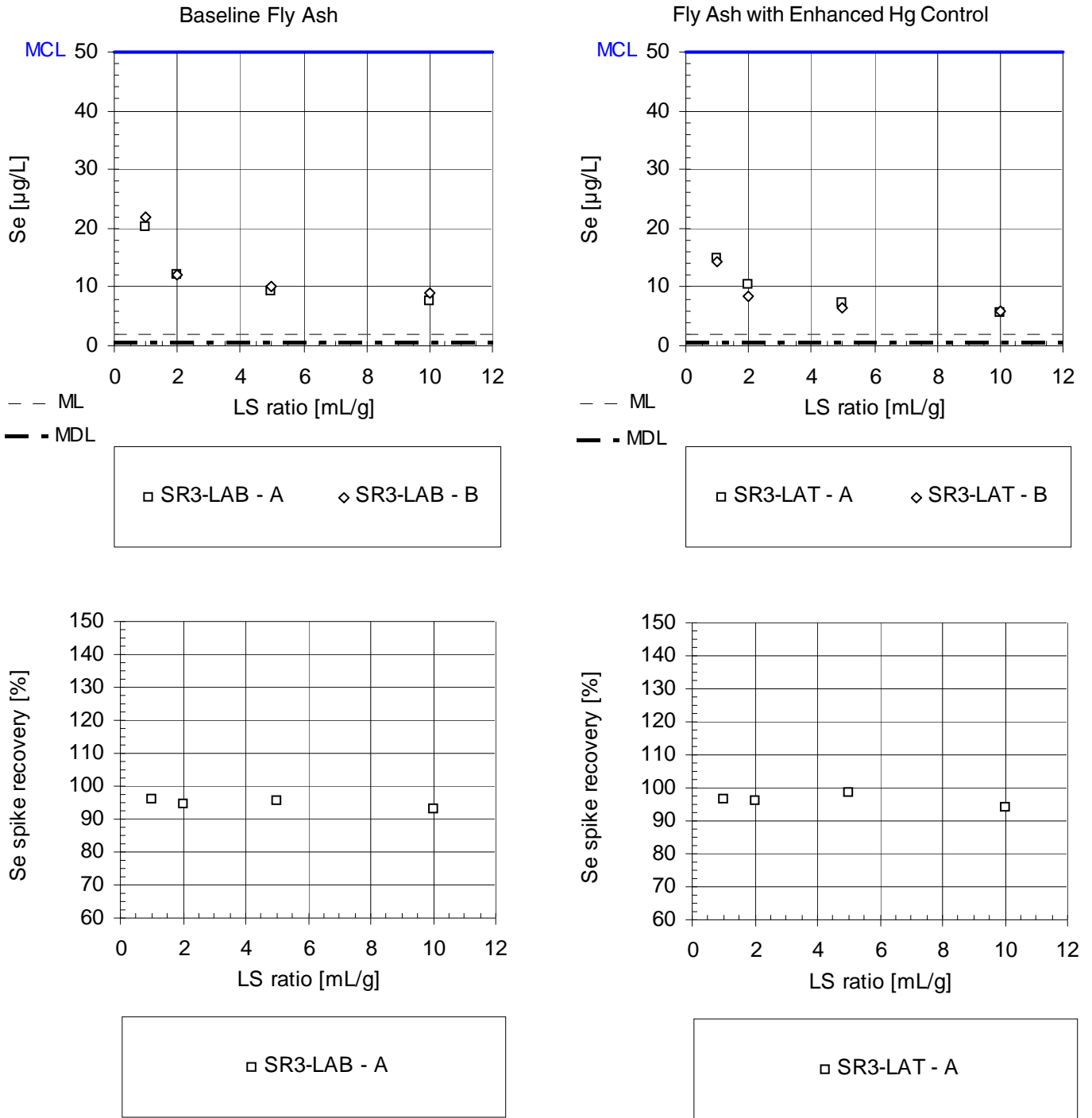
Figure I-8. Selenium Release (top) and Spike Recoveries (bottom) as a Function of LS Ratio for the Baseline Fly Ash and the Fly Ash with Enhanced Hg Control.
