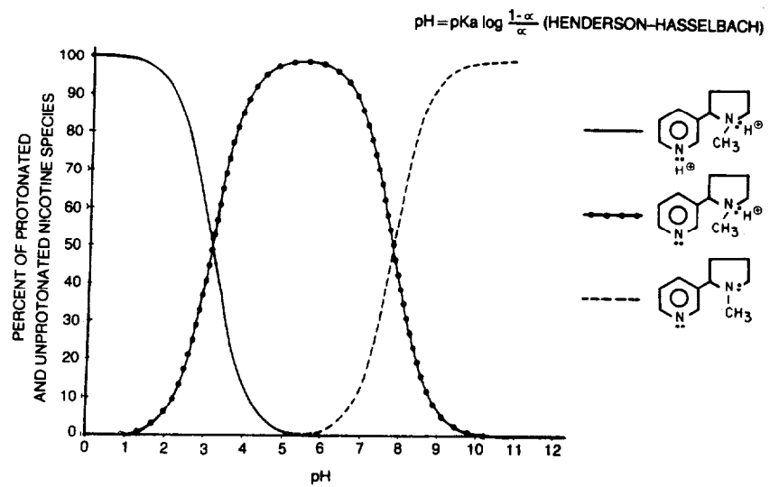
FIGURE 1.—Protonation of nicotine SOURCE: Brunnemann and Hoffmann (28).
