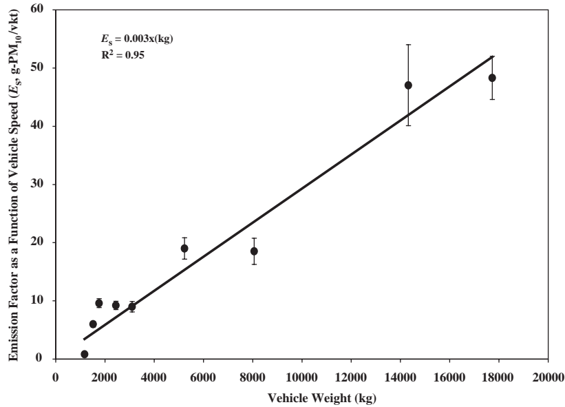
Fig. 6. The slope estimates from the relationship between emission factor and vehicle speed plotted as a function of vehicle weight. The error bars represent the standard error of E_s .
