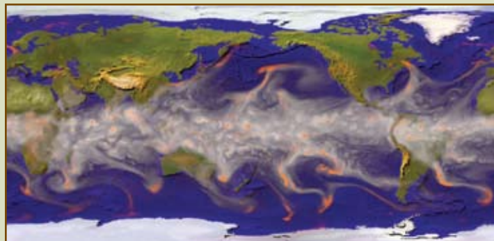
State-of-the-art climate models help researchers to understand and predict global weather patterns and to explore how variables are related.
