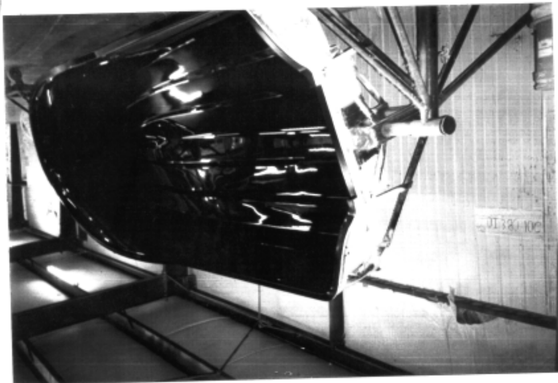
BOW \ STERN VIEW HULL MOLD
