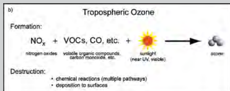
Box Figure 1.2b Schematic representations of the chemical processes that lead to the production and removal of ozone in the troposphere. The VOCs include methane. Other species such as hydrogen also can act as ingredients for ozone production in place of VOCs and CO.
