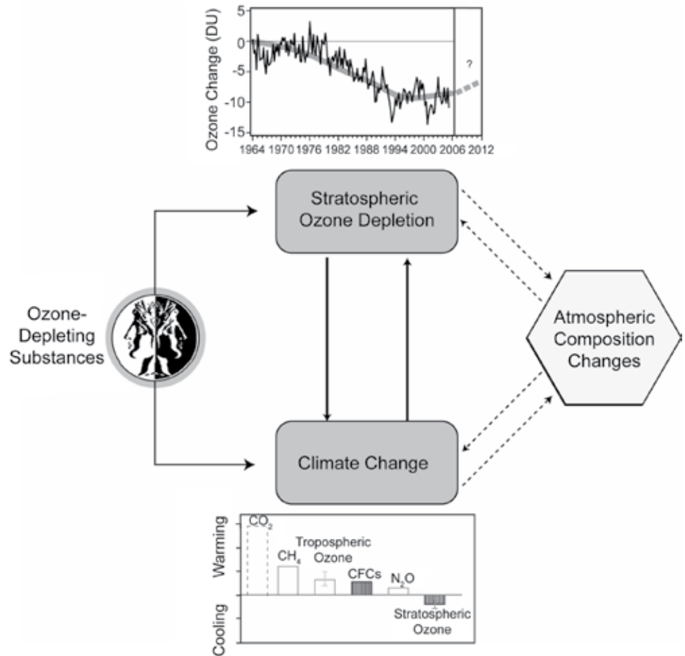
Figure 1.1 The two faces of ozone-depleting substances: their roles as depleting agents of stratospheric ozone, and as greenhouse gases that influence climate. The two roles are further interconnected because ozone itself is a greenhouse gas and because climate change can lead to changes in the ozone layer. The various connections between these two phenomena are shown. A plot of the changes in the observed global ozone illustrates the stratospheric ozone depletion issue. The radiative forcing due to various greenhouse gases, including ODSs, depicts the greenhouse gas issue and stratospheric ozone changes.
