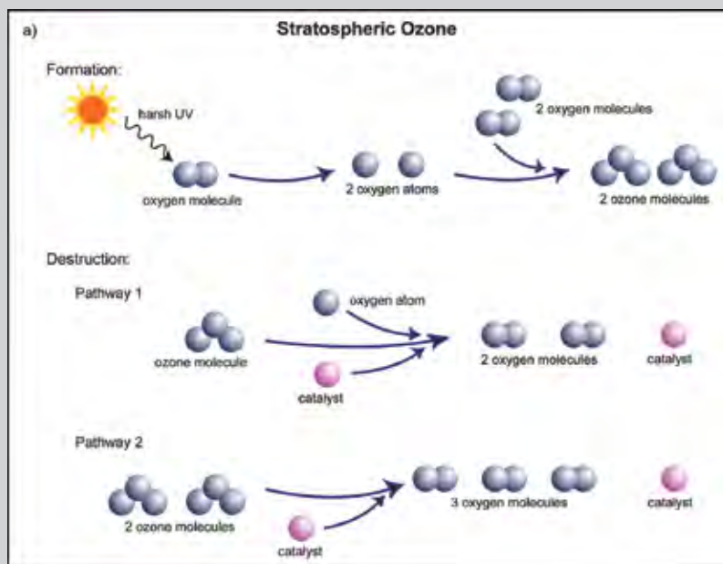
Box Figure 1.2a Highly simplified schematic representation of the chemical processes that lead to the production and removal of stratospheric ozone. The catalysts include both natural and human-emitted species, including chlorine and bromine from ozone-depleting substances. See Chapter 3 and Appendix A for further details.
