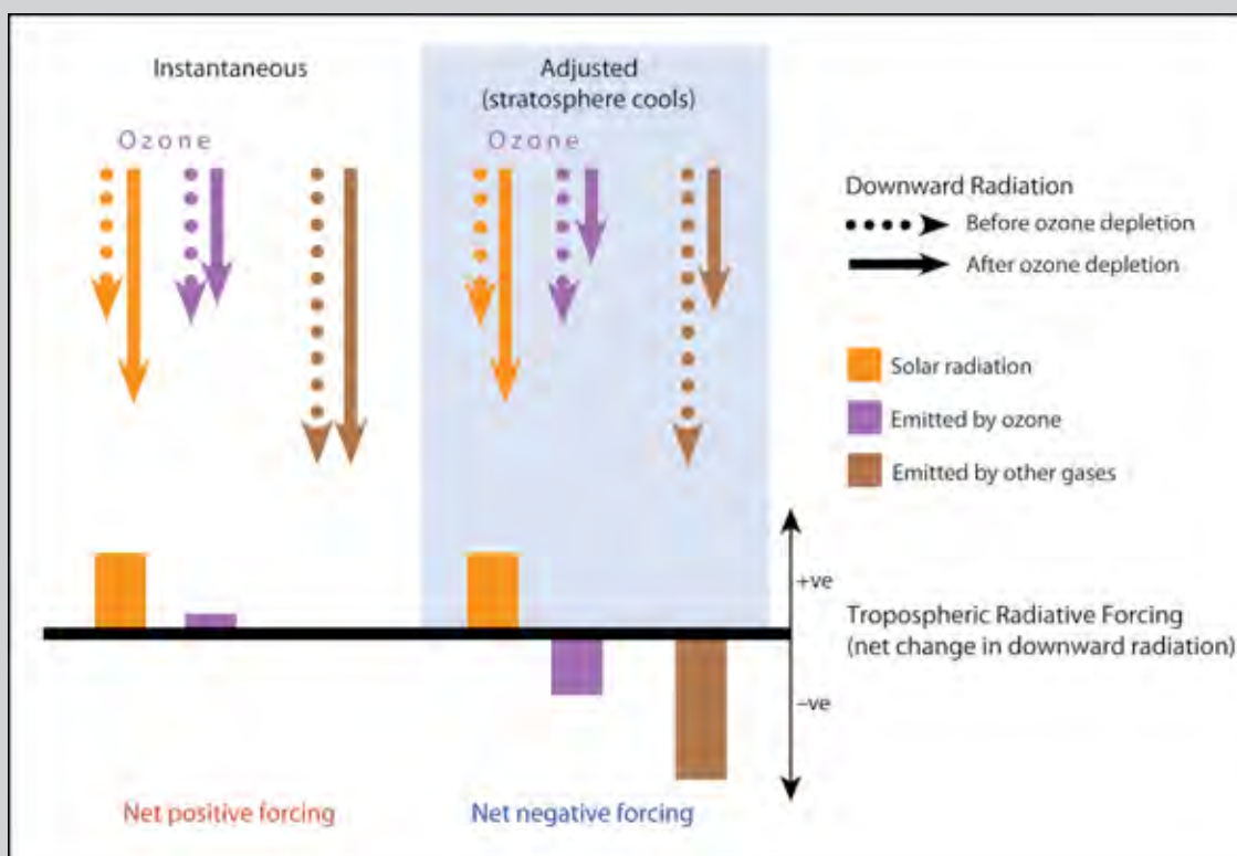
Box Figure 4.2 The instantaneous effect of stratospheric ozone depletion (left-hand side of schematic) is to increase the shortwave radiation from the Sun reaching the tropopause (because there is less ozone to absorb it), and to slightly reduce the downward longwave radiation from the stratosphere, as there is less ozone in the stratosphere to emit radiation. This gives an instantaneous net positive radiative forcing. However, in response to less absorption of both shortwave and longwave radiation in the stratosphere, the region cools, which leads to an overall reduction of thermal radiation emitted downward from the stratosphere (right-hand side of schematic). The size of this adjustment term depends on the vertical profile of ozone change and is largest for changes near the tropopause. For the observed stratospheric ozone changes the adjustment term is larger than the positive instantaneous term, thus the stratospheric ozone radiative forcing is negative.
