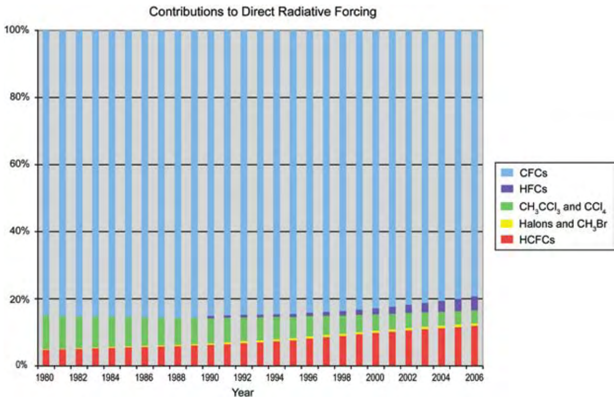
Figure 2.18 Relative contributions of ODS compound classes to global direct radiative forcing. Percentages in 2005 are CFCs=80%, HCFCs = 12%, other ODSs = 5%, HFCs = 4%.
