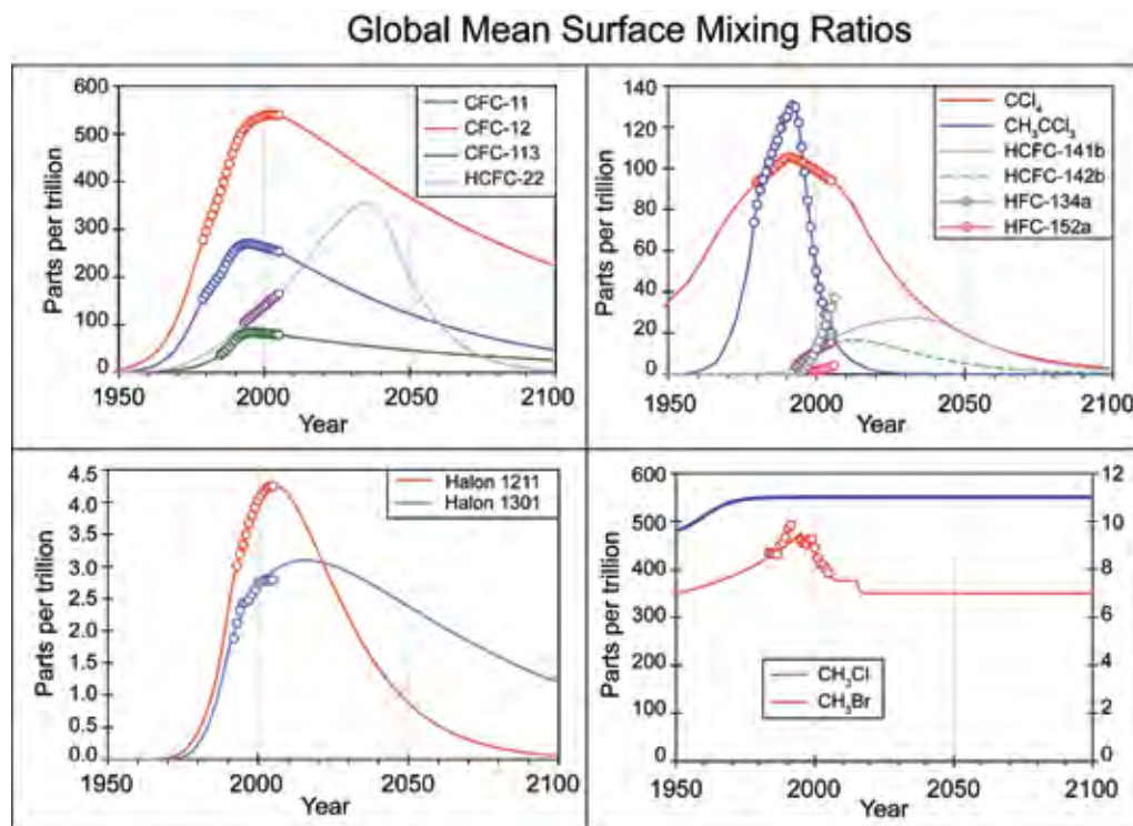
Figure 2.12 Global surface mixing ratios of ODSs and substitute chemicals observed from surface sampling networks (open circles), and as estimated for the past and future in WMO scenario AI (Clerbaux and Cunnold et al. , 2007; Daniel and Velders et al. , 2007). Past projections are based on histories derived from the analysis of archived air samples, the analysis and modeling of firn-air (air trapped in uncompacted snow in the polar regions) samples, and historic industrial production data.
