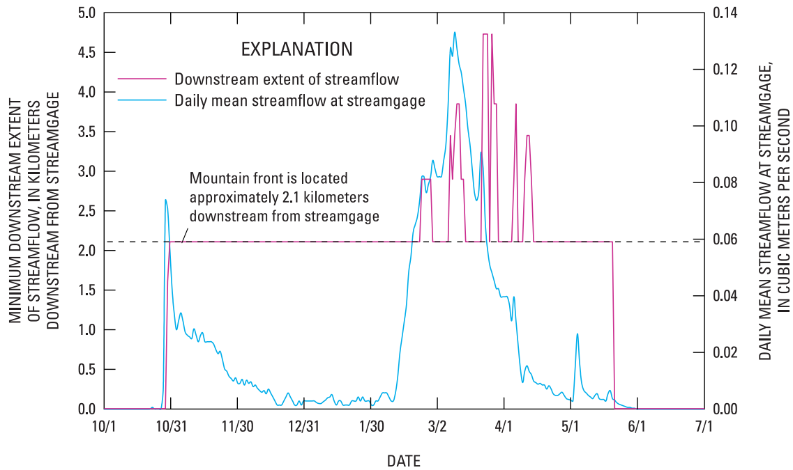
Figure 7. Minimum downstream extent of seasonal streamflow in Arroyo Hondo, New Mexico, compared with the daily mean streamflow at the upstream streamflow station (USGS gage 08317050) over the 2000–2001 seasonal streamflow season [from Moore, 2007].
