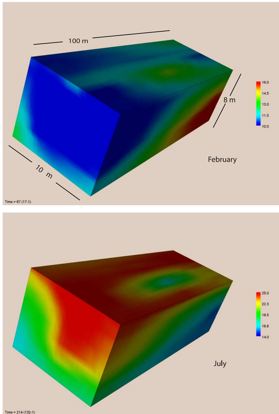
Figure 11. A pair of instantaneous 3-D streambed TC plots for early February and early July 2004 beneath a flowing reach of the Consumnes River, California, based on interpolation of a series of thermocouple cross-sections. The upper surface of TC plots denotes the streambed surface, with the stream residing above this surface, flowing from the upper right corner toward the left along the 100-m axis (modified from Niswonger [2005]).
