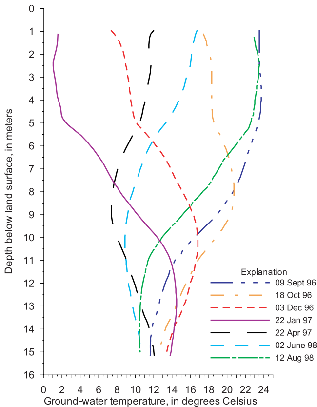
Figure 8. Temperature envelopes for the streambed of the Rio Grande, New Mexico, collected beneath the right (west) bank from September 1996 through August 1998 to a depth of 15 m below the elevation of the streambed surface (modified from Bartolino and Niswonger [1999]).
