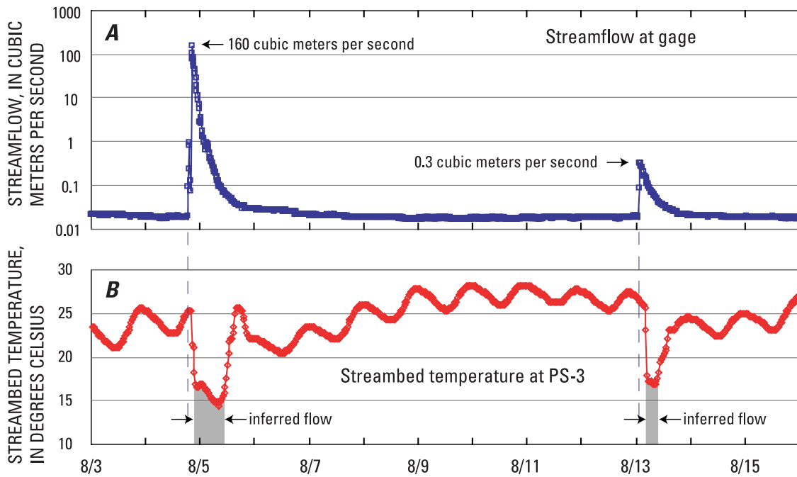
Figure 6. (a) Streamflow hydrograph at Abo Arroyo (USGS gage 08331660) and (b) streambed thermograph at a probe site 2.6 km downstream, 3–16 August 1998. Shaded areas on the thermograph indicate periods of inferred streamflow reaching the probe site [from Stewart et al. , 2007].
