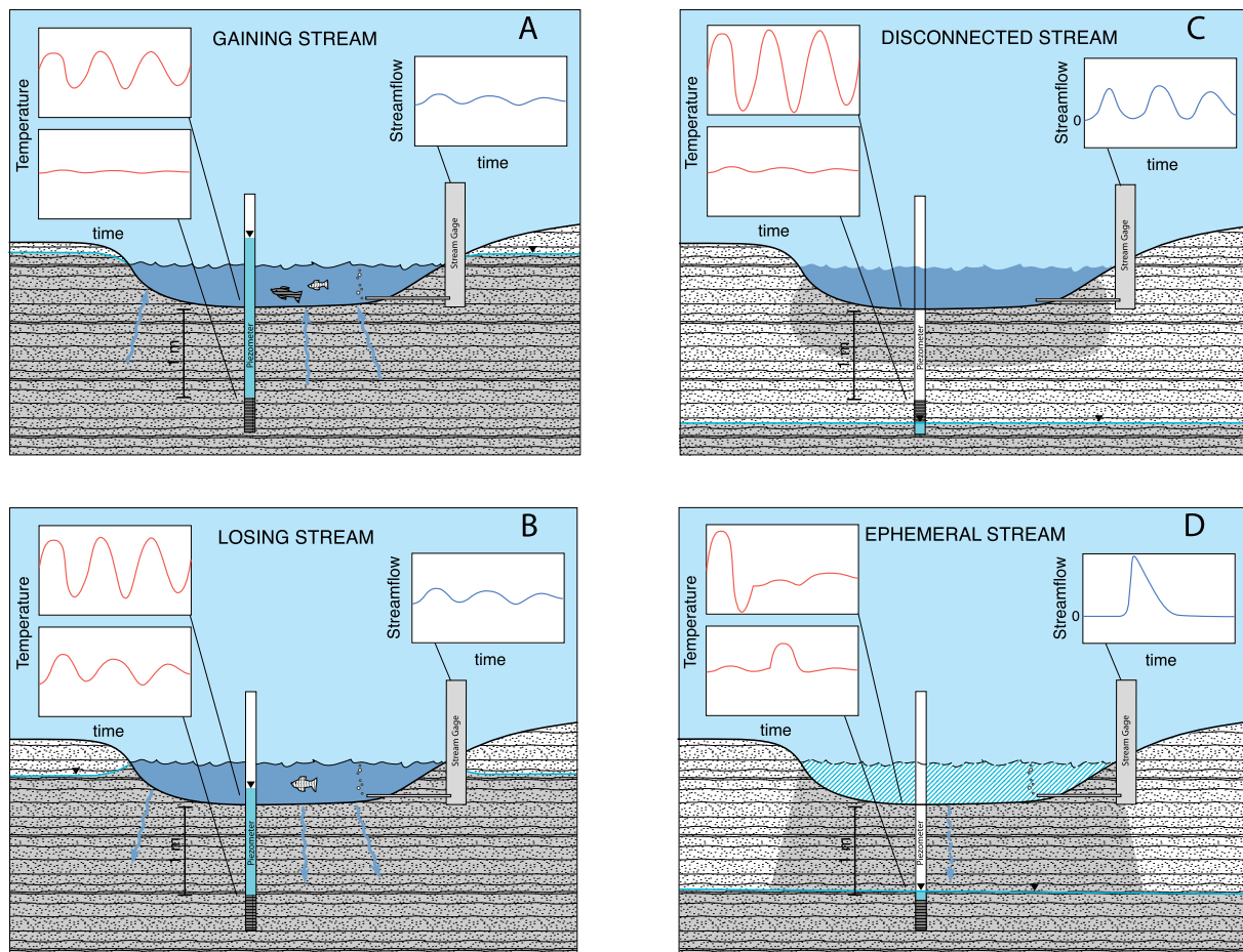
Figure 2. Thermal and hydraulic conditions in streambeds under the influence of streamflow for (a) gaining, (b) losing, (c) disconnected, and (d) ephemeral stream settings. Inset plots of thermographs and hydrographs are located in the upper left and right panels of the figure (modified from Constantz [2008]).
