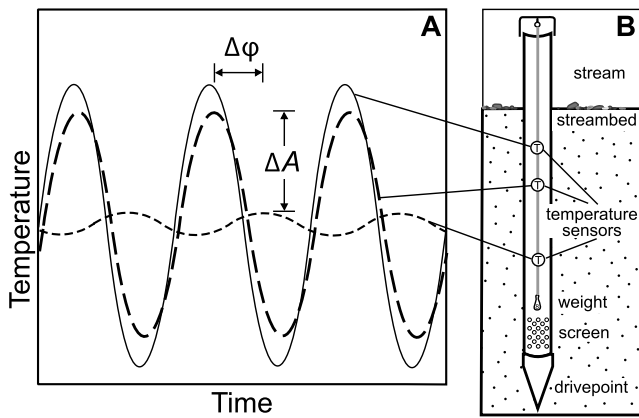
Figure 3. (a) Three hypothetical streambed thermographs graphed over three days, showing phase shift ( \Delta\phi ) and difference in temperature amplitude ( \Delta A ), and (b) a typical temperature acquisition assembly inside a piezometer (modified from Hatch et al. [2006]).
