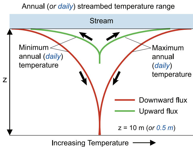
Figure 4. Hypothetical temperature envelopes depicting the extreme high and low annual (or daily) temperature profiles propagating downward into homogeneous sediments from the streambed surface in the absence of nonvertical flow components (modified from Constantz and Stonestrom [2003]).
