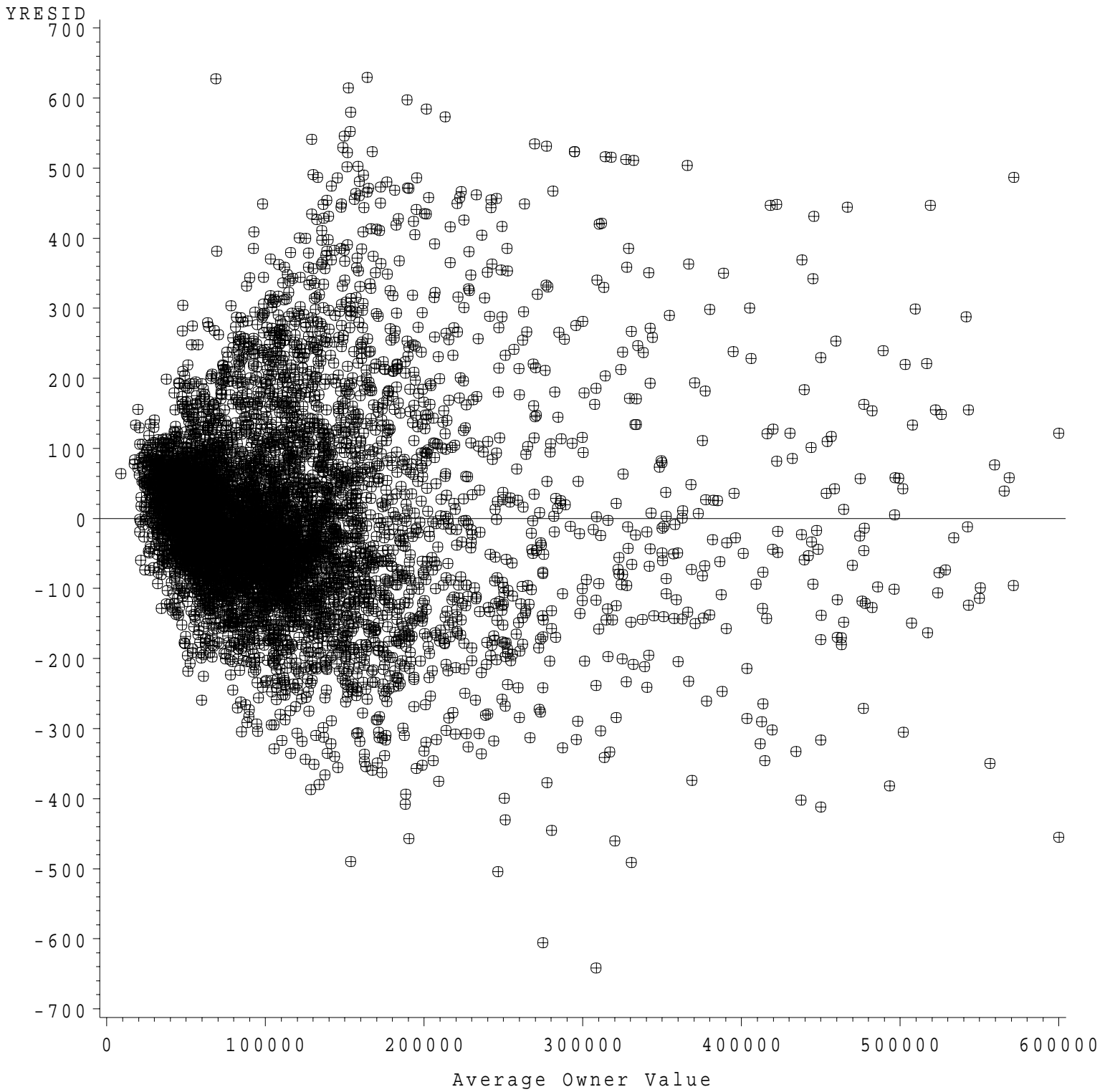
Figure 3.3 Plot of residuals of exponential function
