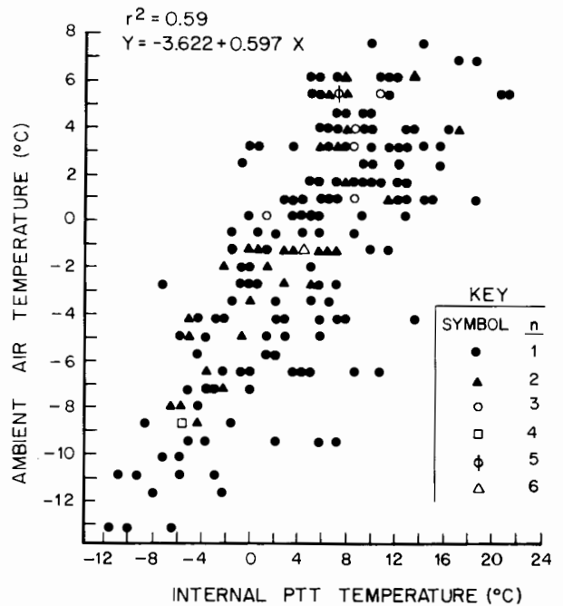
Fig. 26. Relation between ambient temperature and the internal temperature of the platform transmitter terminal (PTT) canister (adapted from Pank et al. 1985).
