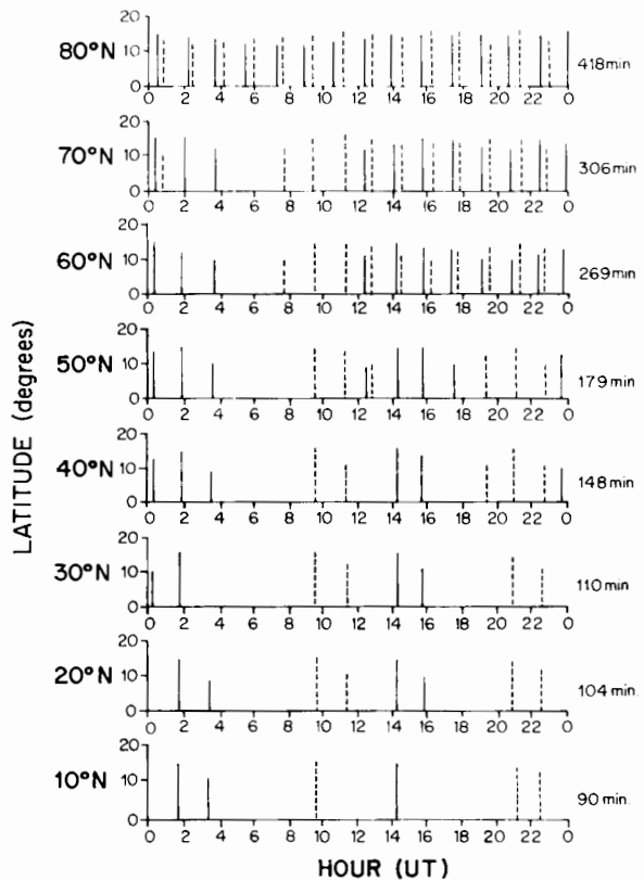
Fig. 10. Daily frequency and duration of overpasses by NOAA-9 (dashed lines) and NOAA-10 (solid lines) at various latitudes. The exact time and duration of each overpass varies, but the general pattern of satellite coverage is similar each day. Numbers on the right give the total time a satellite is above the horizon at each latitude. At higher latitudes a single transmitter may be within view of two satellites simultaneously.
