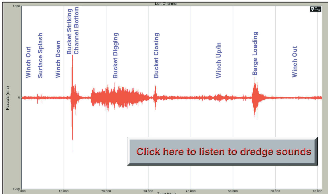
Figure 3. An example pressure waveform for a typical bucket deployment and retrieval cycle
