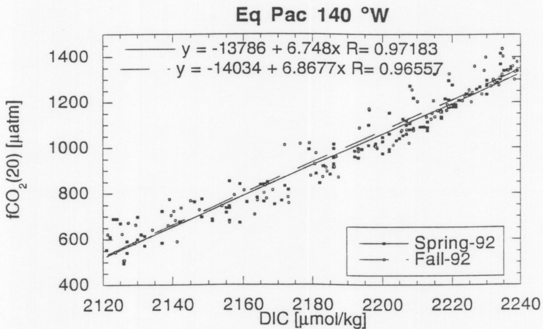
Figure 29. Top: pH plotted against DIC for intermediate waters with DIC content between 2120 and 2240 \mu\text{mol kg}^{-1} for EqPac spring and fall-92. Bottom: fCO 2 (20) plotted against DIC for intermediate waters with DIC content between 2120 and 2240 \mu\text{mol kg}^{-1} .
