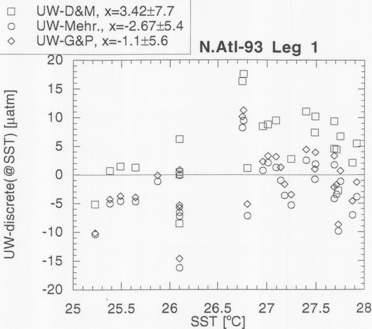
Figure 7. Influence of carbon dissociation constants on temperature correction to convert f\text{CO}_2(20) to f\text{CO}_2 at SST. The difference between the underway measurements and the temperature corrected discrete f\text{CO}_2 values are plotted against temperature for data obtained during the N.ATL-93 cruise, leg 1. D&M=carbon dissociation constants of Dickson and Millero [1987]; Mehr.= constants of Mehrbach [1973], and G&P= those of Goyet and Poisson [1989].
