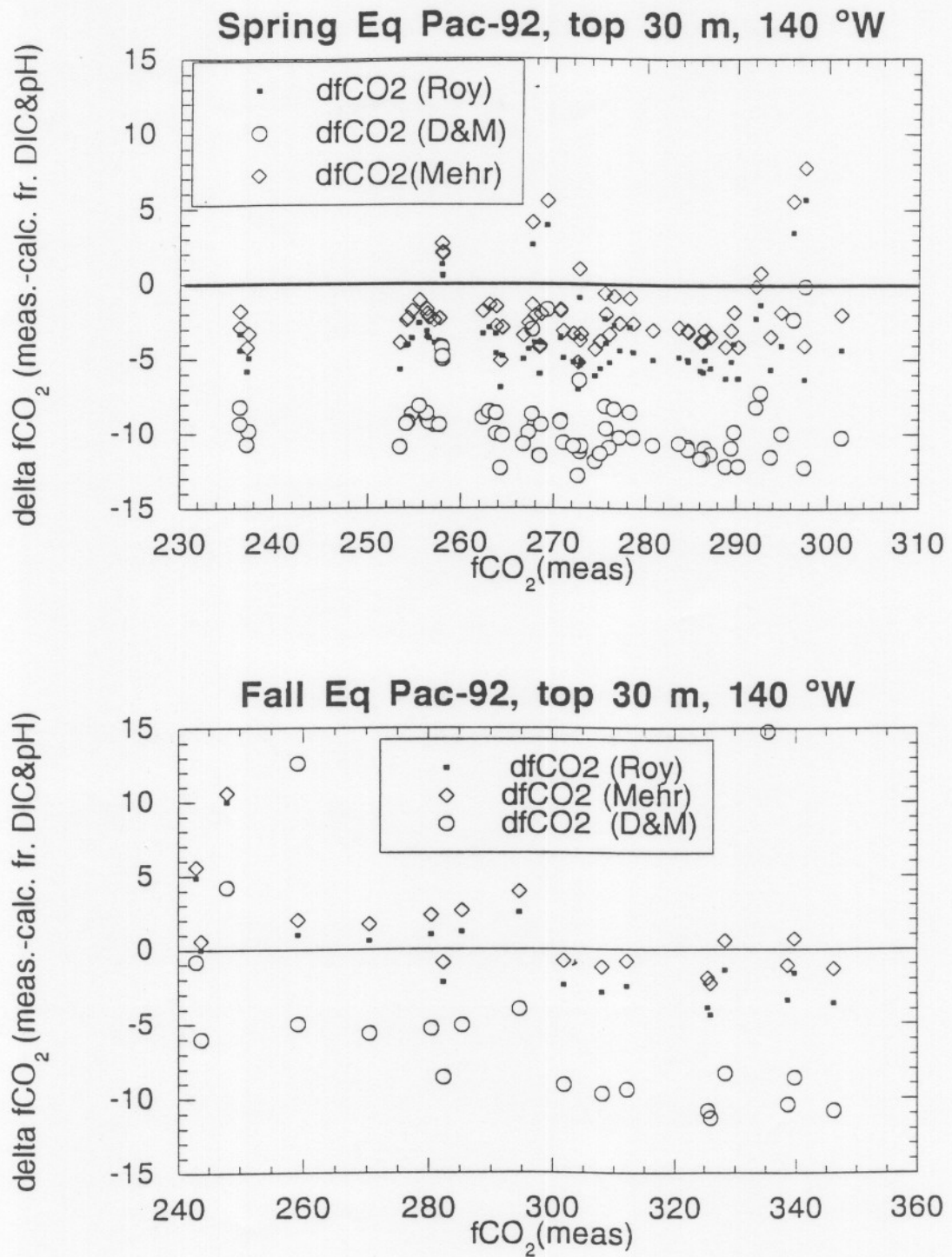
Figure 30. Difference of measured fCO 2 (20) and calculated fCO 2 (20) from DIC and pH, for samples in the surface mixed layer (0-30 m) for EqPac spring and fall-92.
