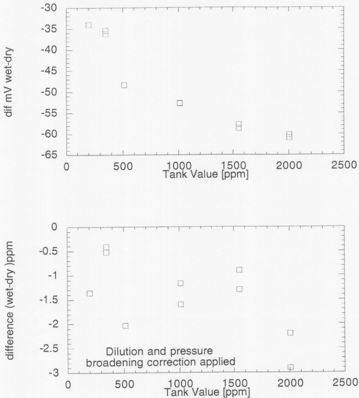
Figure 4. Top: Difference in response of the IR detector to dry and water saturated (20 °C) standard gases. Bottom: Difference in response (in ppm) after the instrumental water vapor correction is applied to the moist gas, illustrating that the correction is quite robust. Note that in our work we do not rely on either the instrumental water vapor correction or internal conversion from detector response (in mV) to mixing ratio.
