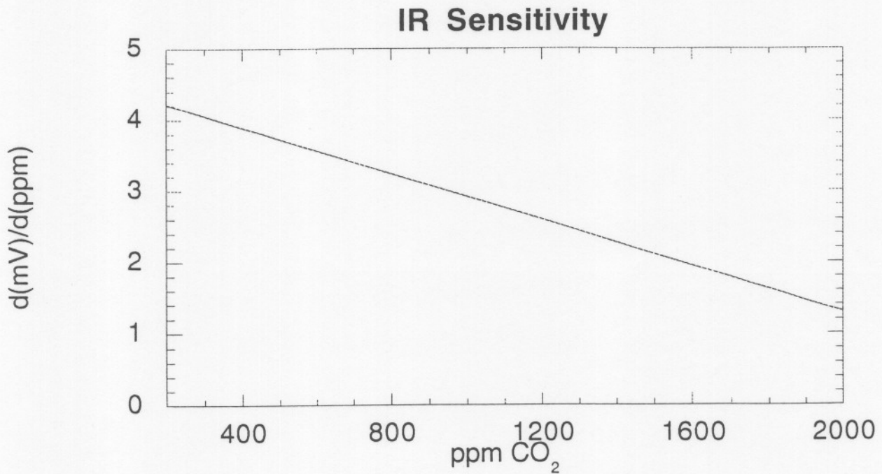
Figure 2. Top: typical response curve of the IR detector to different gas standards. Bottom: change in response with increasing concentrations. Note the fourfold decrease in sensitivity over the operational range of the IR detector.
