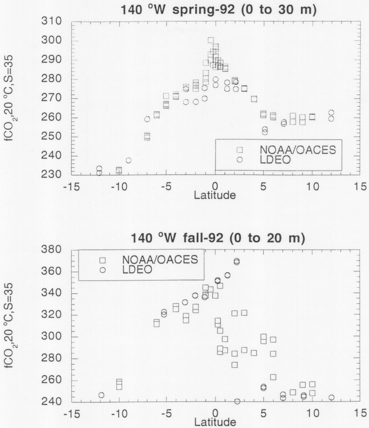
Figure 13. Comparison of EqPac spring and fall-92 surface water f\text{CO}_2(20) normalized to S=35 with f\text{CO}_2(20) obtained along the same ( 140^\circ\text{W} ) transect by LDEO during the same season and year but about 1.5 months earlier for the (boreal) spring and 2 weeks later for the fall.
