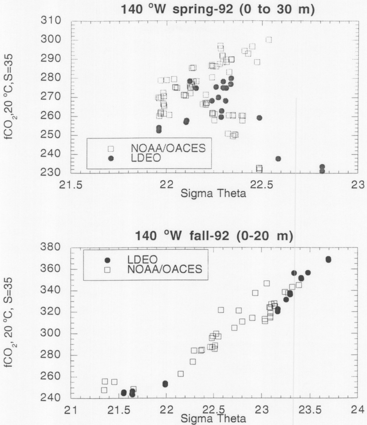
Figure 14. Comparison of EqPac spring and fall-92 surface water f\text{CO}_2(20) normalized to \text{S}=35 with f\text{CO}_2(20) obtained along the same ( 140^\circ\text{W} ) transect by LDEO during the same season and year. The surface water data is plotted against potential density.
