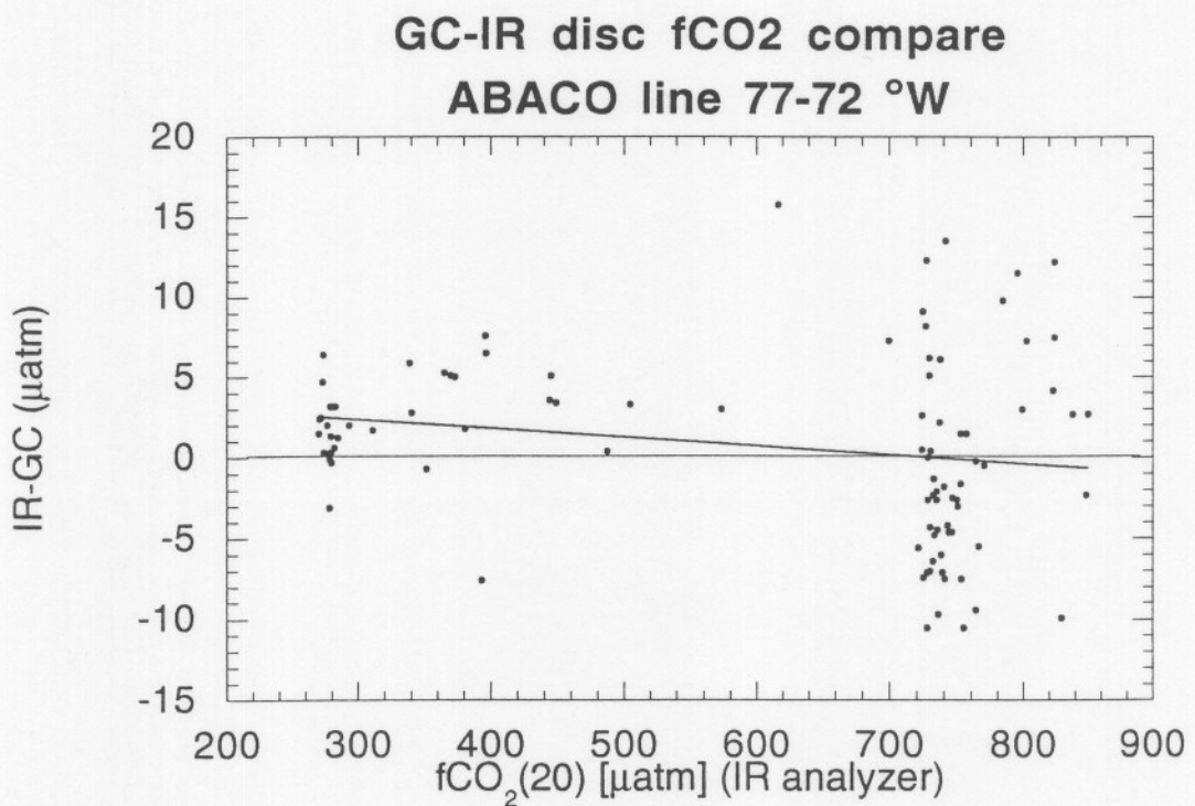
Figure 9. Differences in f\text{CO}_2(20) obtained with the IR analyzer system described and a recently fabricated GC based system. Top: a composite plot of all samples taken from 11 stations along the ABACO line (77 °W to 72 °W, 26.5 °N). Bottom: Difference in IR analyzer and GC based measurements from samples taken from the same Niskin™ bottle plotted against f\text{CO}_2(20) .
