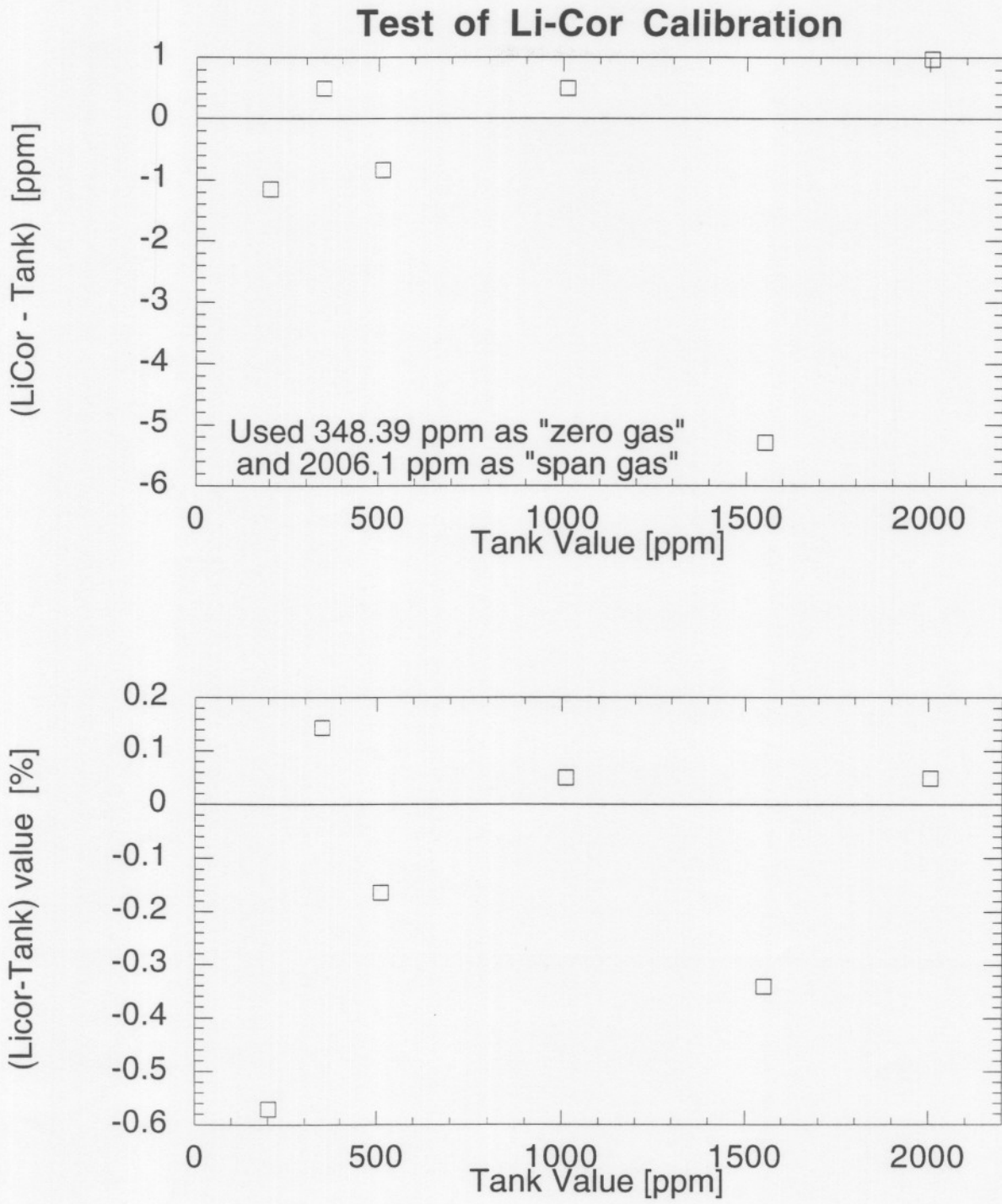
Figure 3. Top: comparison of the internal calibration of the IR detector and the absolute tank calibration, expressed as the difference between the LI-COR IR detector value and the tank value (calibrated against WMO referenced gases). This example illustrates that the empirical algorithm supplied with the detector is quite accurate. Bottom: same as top figure except expressed as percent of the corresponding standard value
