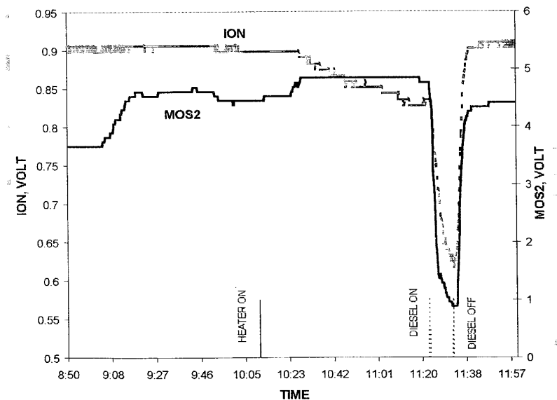
Figure 3—This graph illustrates the sensors response to a smoldering coal fire and diesel exhaust at a battery-charging station.
