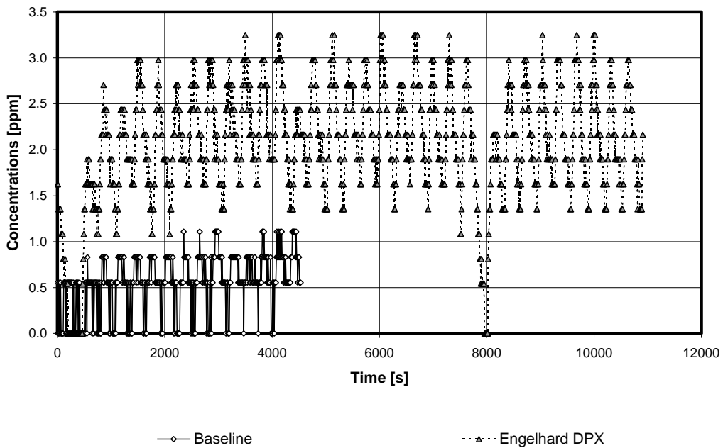
Figure 32.—Normalized NO 2 concentrations at the downstream sampling station for the tests with haul truck #92128.
