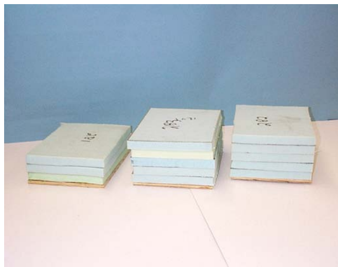
Figure 5.—Viscoelastic arrangements for the low-coal-seam shuttle car seat.
