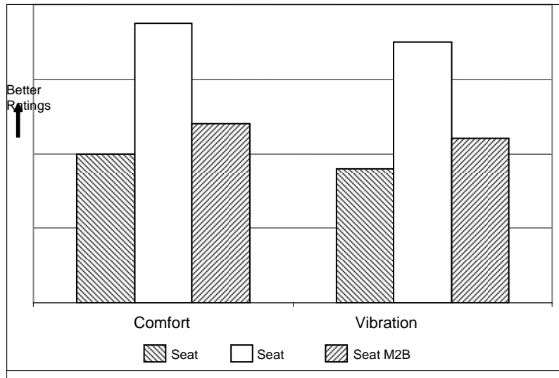
Figure 10.—Seat ratings of mid-coal-seam shuttle car operators on comfort and vibration reduction.
