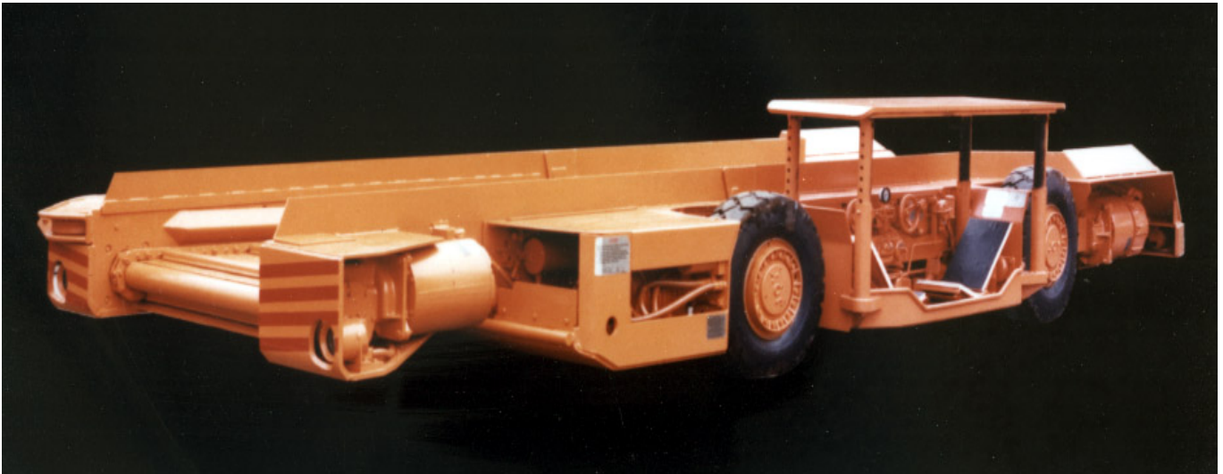
Figure 1.—JOY 21SC low-coal-seam shuttle car.
