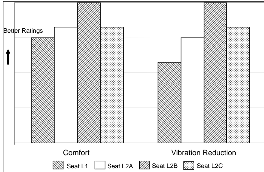
Figure 13.—Low-coal-seam shuttle car operators' ratings of seat designs for comfort and vibration reduction.
