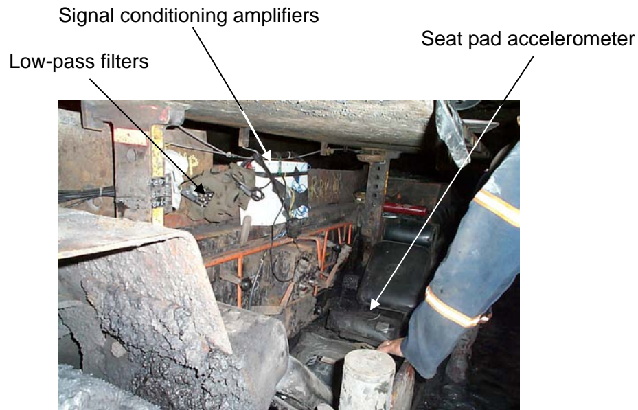
Figure 9.—Instrument setup on the low-coal-seam shuttle car seat.
