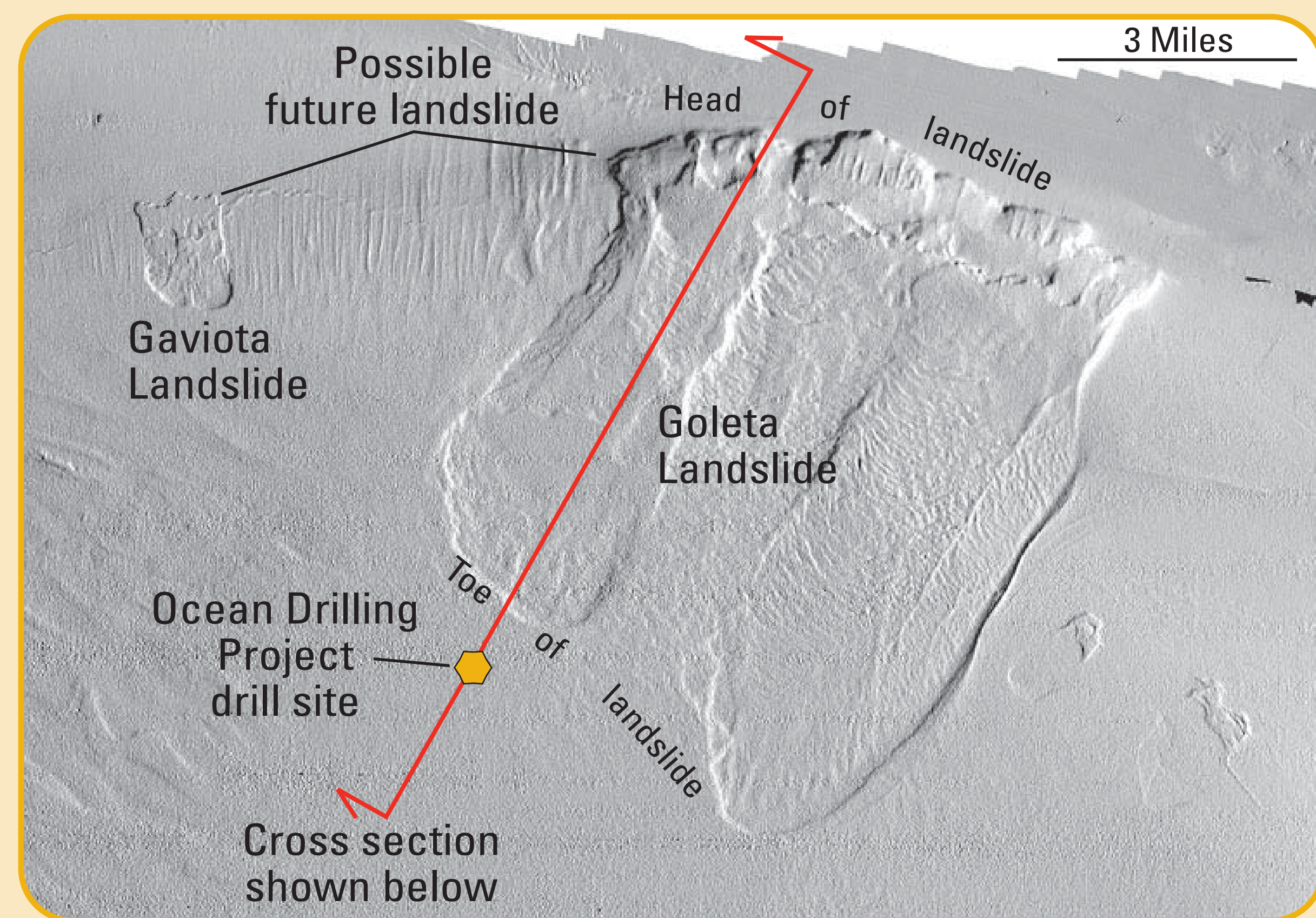
Underwater landslides offshore from Santa Barbara.
