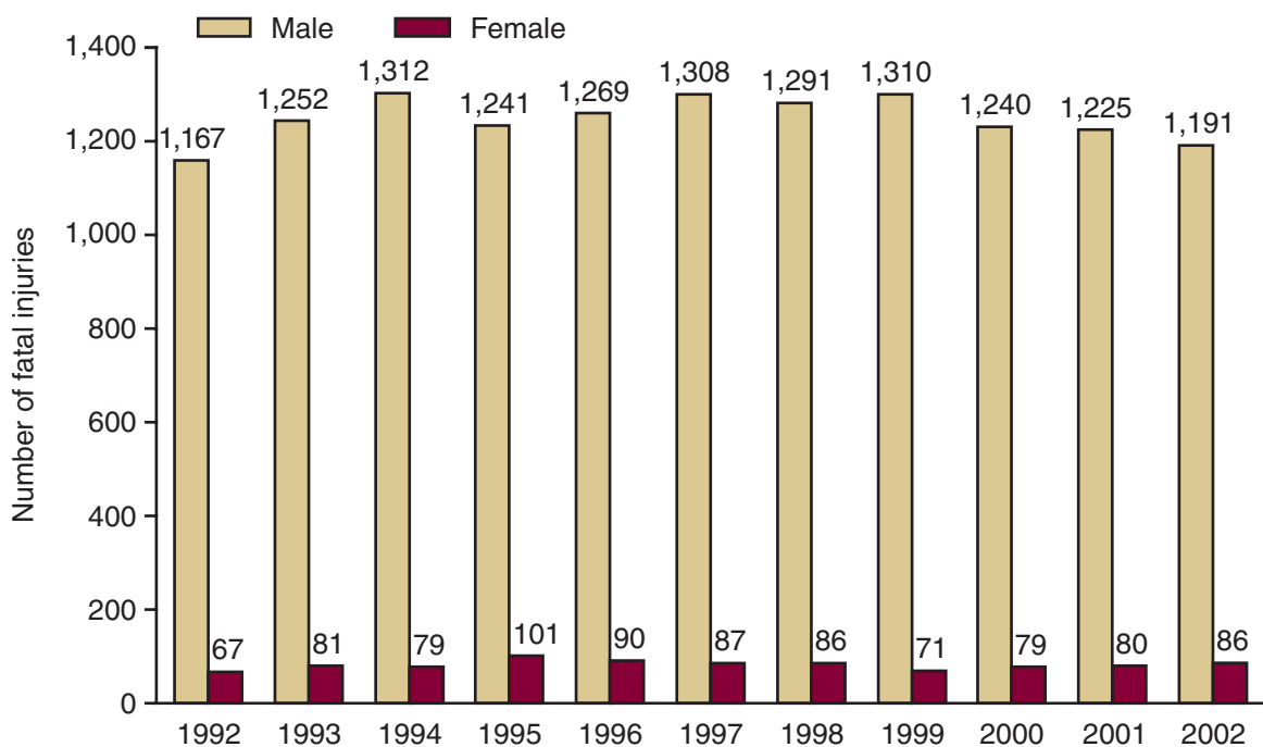
Figure 5–23. Number of fatal occupational injuries among workers aged 55 and older by sex, 1992–2002. Male workers accounted for most fatal occupational injuries among older workers (94% during the 11-year period). From year to year, small differences occur in the number of fatal injuries among women, ranging from 67 in 1992 to 101 in 1995. (Source: BLS [2003d].)
