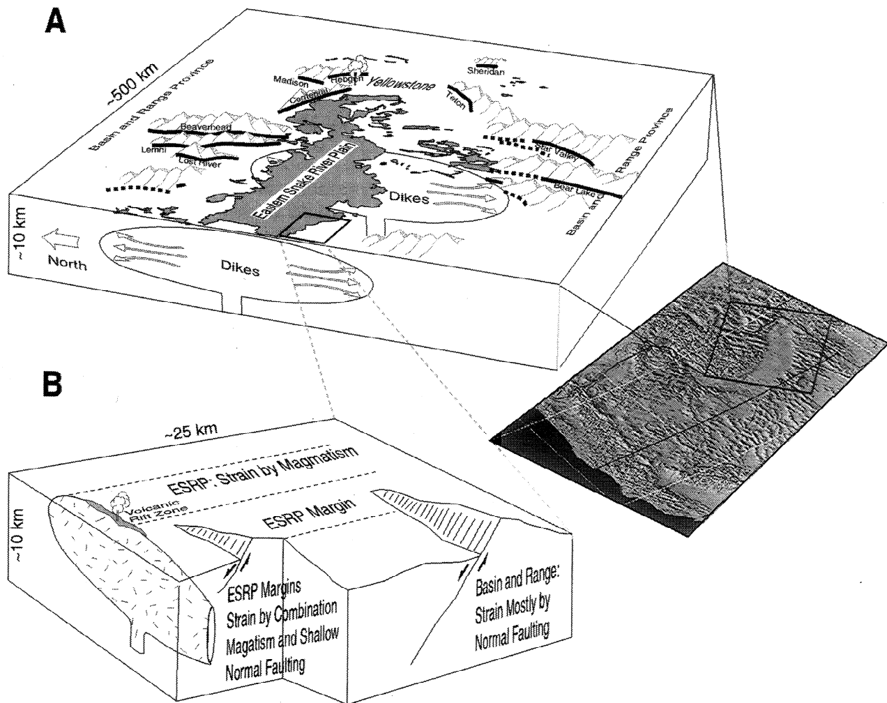
Figure 5. Proposed model for the aseismic elastic strain of the eastern Snake River Plain and transitional behavior of the transition zone of the plain. (a) Regional sketch showing on and off axis volcanism with underlying feeder dike complexes inferred from volcanic rift zones, magnetic anomalies, and the existence of young vents off the central axis of the plain. The dikes are meant to be symbolic in the sketch and are understood to be far more complex than shown [e.g., Kuntz et al. , 1992]. (b) Close up sketch showing the proposed variable role of magmatic strain. Within the eastern Snake River Plain we suggest dikes are the primary strain mode because (1) of the lack of developed fault-block morphology, (2) only microearthquakes occur within the plain (magnitudes < 1.5 [e.g., Jackson et al. 1993]), (3) in situ stress indicators find low deviatoric stresses [Moos et al. , 1990], and (4) of the presence of abundant flood basalts and volcanic rift zones on the plain. Within the transition zone of the plain, highly variable seismicity, ages of fault slip, reduced fault spacing and earthquake focal depths (compared with Basin and Range averages), and variable occurrences of magmatism indicate a transition from magmatic to normal-fault extensional strain. Away from the transition zone, normal faulting becomes the primary strain mode, possibly enhanced by deep-seated isostatic effects caused by the Yellowstone plume [e.g., Anders and Sleep, 1992; Pierce and Morgan, 1992].
