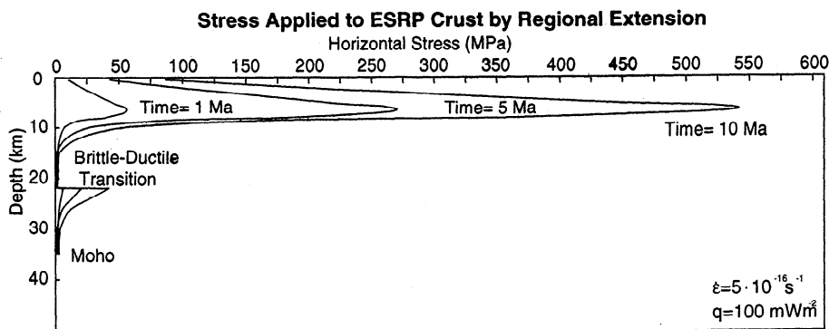
Figure 2. Theoretical build-up of differential stress in the brittle upper eastern Snake River Plain crust if the rocks are strong enough to resist regional extensional strain over time periods of 1, 5, and 10 m.y. The lithosphere is treated as a Maxwell viscoelastic solid where stress and strain are linked through the equation \epsilon_x = \frac{1}{E}(\sigma_x - \sigma_x^0) - \frac{\nu}{E}(\sigma_y - \sigma_y^0) - \frac{\nu}{E}(\sigma_z - \sigma_z^0) + \epsilon_x^v , where \epsilon is strain ( \epsilon_x^v is ductile creep in the x direction), \sigma is stress ( \sigma_x^0 is initial stress), E is Young's modulus, and \nu is Poisson's ratio (see Kusznir and Park , [1984,1987] for complete details on the method). Applying a strain rate of 5.0 \times 10^{-16} \text{ s}^{-1} over time yields extremely high stresses in the upper crust that far exceed the observed 1-to 10-MPa stress drop for normal-fault earthquakes [e.g., Kanamori and Anderson , 1975; Jackson and Blenkinsop , 1993].
