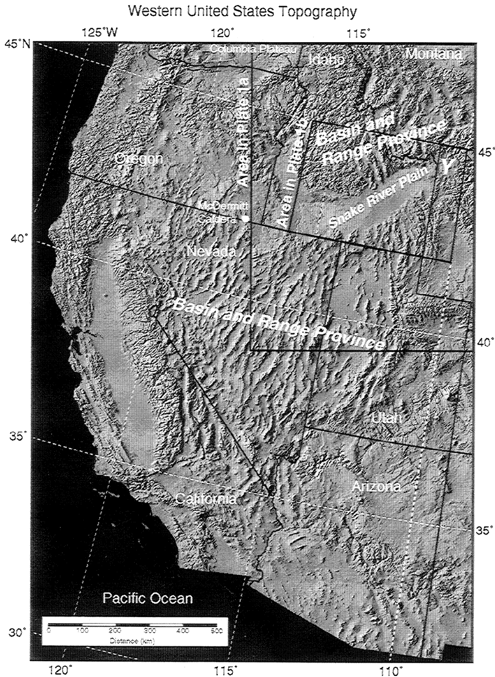
Figure 1. Topography of the Basin and Range Province [Thelin and Pike, 1991]. The low-relief Snake River Plain is one of the most distinctive topographic features of the province. Yellowstone is marked by the letter, "Y". Rectangles show the areas covered in Plates 1a and 1b.
