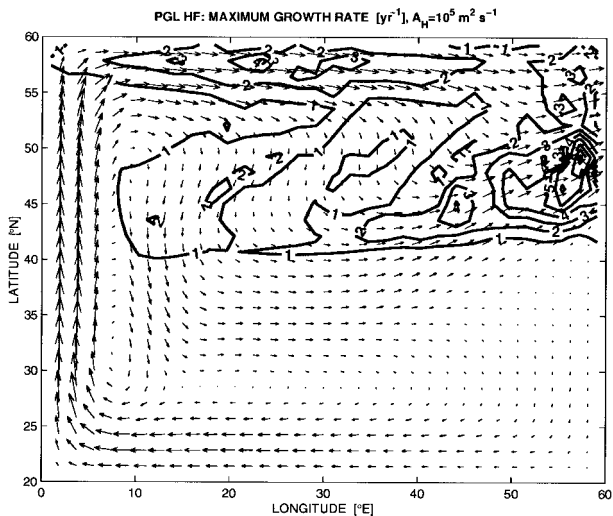
FIG. 4. Maximum growth rate of baroclinic instability ( \text{yr}^{-1} ) at each horizontal location for the time-averaged vertical profiles of density and velocities of the coarse-resolution model (L160) with a viscosity of 10^5 \text{ m}^2 \text{ s}^{-1} . The arrows are the time-averaged model velocities in the upper 250 m, the scale is 2 \text{ cm s}^{-1} per degree of latitude or longitude.
