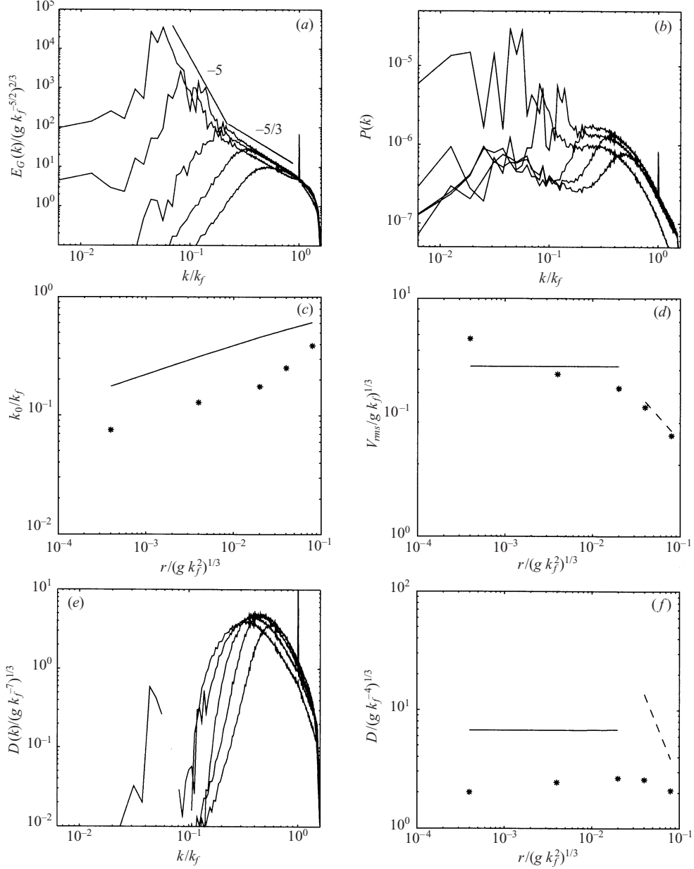
FIGURE 8. Same as figure 2 but TDV flow with varied drag and fixed \beta^* = 0.73 . Values of drag used are r^* = (0.040, 0.43, 2.1, 4.3, 8.5) \times 10^{-2} , and the critical drag of (6.7) is r_c^* = 9.0 \times 10^{-2} . The effective generation rates are g_{eff} = 0.35, 0.37, 0.42, 0.54, 0.60 . Theoretical predictions are discussed in § 7.4. Missing values in (e) are negative but small. Dashed lines in (d) and (f) represent predictions for large-drag, \beta = 0 limit.
