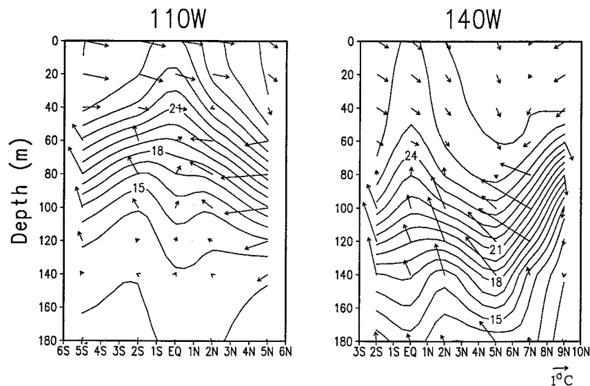
FIG. 4. The annual mean temperature along 110°W and 140°W. The contour interval is 1°C. The arrows indicate the amplitude and phase of the annual harmonics at locations where measurements are available. The length of an arrow corresponds to the amplitude. The length of the arrow in the right lower corner is 1°C. The direction of an arrow represents the phase. An upward pointing arrow indicates that the maximum of the annual cycle occurs in January, and a rightward pointing arrow indicates that the maximum of the annual cycle occurs in April.
