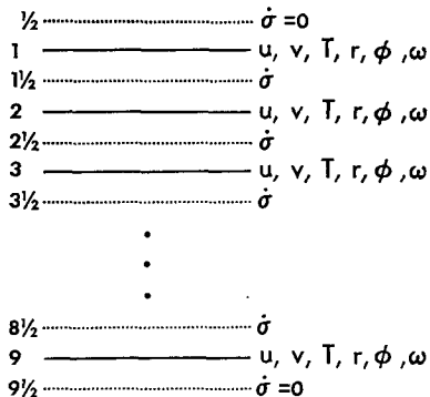
FIG. 2. The indexing scheme for the vertical finite differencing.
