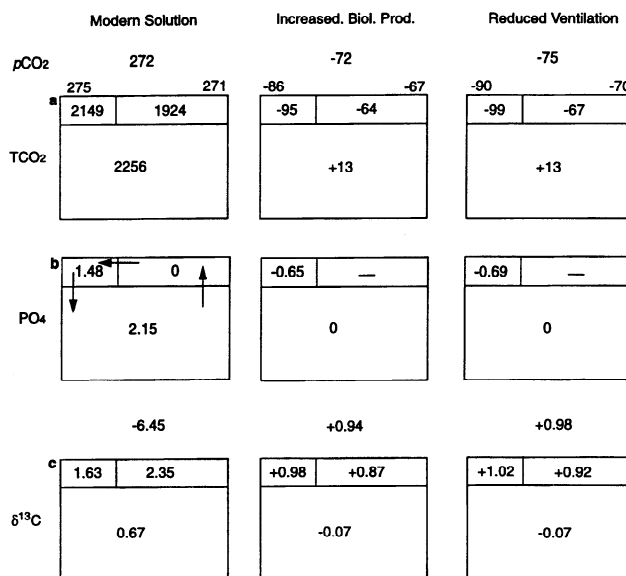
Figure 3. Solutions of the three-box model for (a) p\text{CO}_2 and total CO 2 concentrations (TCO 2 ), (b) PO 4 , and (c) δ 13 C for a high-CO 2 modern state (in the left column, f_{hd} = 60 Sv and P_h = 1.0 moles C m -2 yr -1 ) and two low-CO 2 states (middle and right columns). The low-CO 2 state in the middle is produced by increasing P_h to 6.3 moles C m -2 yr -1 with f_{hd} constant. The low-CO 2 state on the right is produced by reducing f_{hd} to 19 Sv with P_h constant. Results for the two low-CO 2 states are given as differences from the high-CO 2 state. The increase in P_h and reduction in f_{hd} are the only changes being made to reduce atmospheric CO 2 , no changes have been made to reflect colder glacial temperatures, a higher salinity, or a smaller terrestrial biosphere. The alkalinity difference between the d box and the l box is nearly the same in all three solutions, 107.5 μeq kg -1 .
