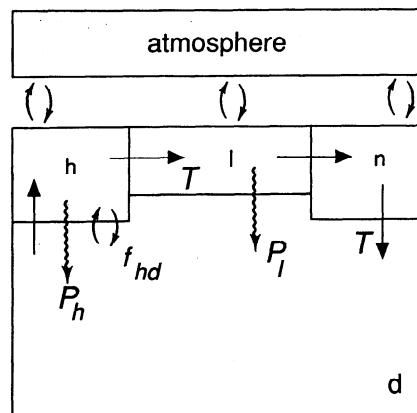
Figure 4. Schematic diagram of the four-box model.
