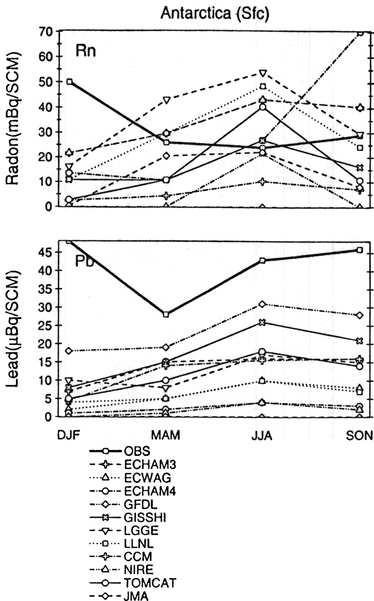
Fig. 6. Seasonal variations in radon and lead over Antarctica for the models (various thin line patterns) and the observational estimate (as the heavy black line).
